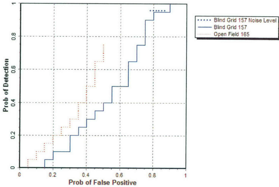
Figure 8. EM61 MKII response stage probability of detection ( P_d^{res} ) versus the respective probability of false positive ( P_{fp} ) for ordnance larger than 20 mm.
