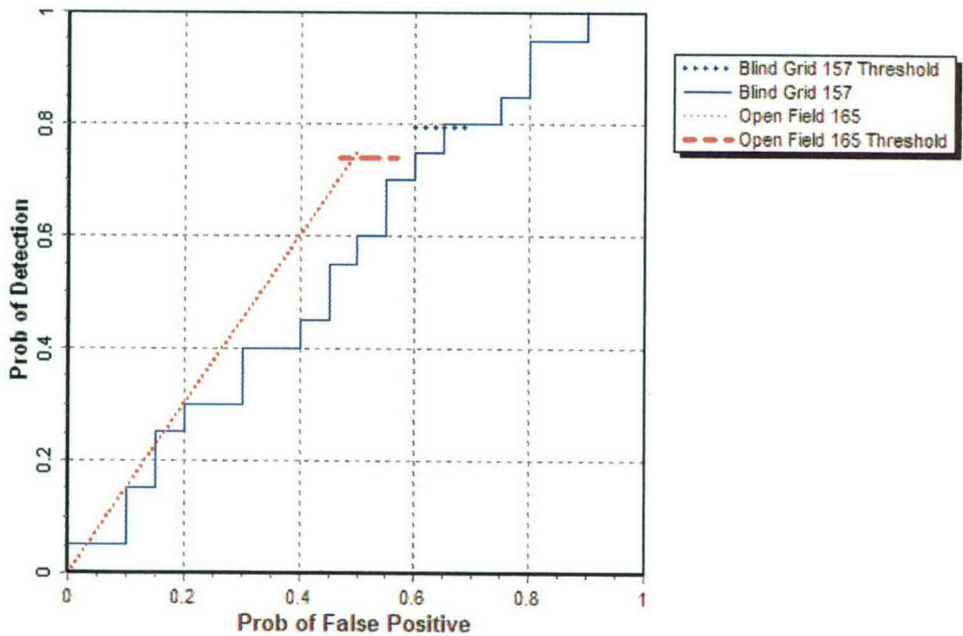
Figure 9. EM61 MKII discrimination stage probability of detection ( P_d^{disc} ) versus the respective probability of false positive ( P_{fp} ) for ordnance larger than 20 mm.
