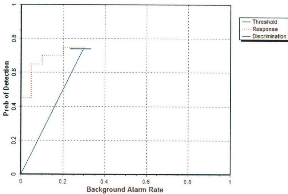
Figure 5. EM61 MKII open field probability of detection for the response stage ( P_d^{\text{res}} ) and the discrimination stage ( P_d^{\text{disc}} ) versus their respective probability of background alarm response ( BAR^{\text{res}} ) for all ordnance larger than 20 mm.
