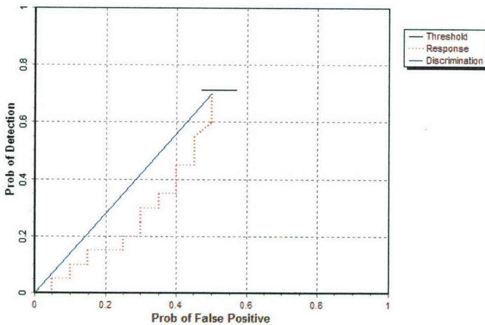
Figure 2. EM61 MKII open field probability of detection for the response stage ( P_d^{\text{res}} ) and the discrimination stage ( P_d^{\text{disc}} ) versus their respective over all ordnance categories combined.
