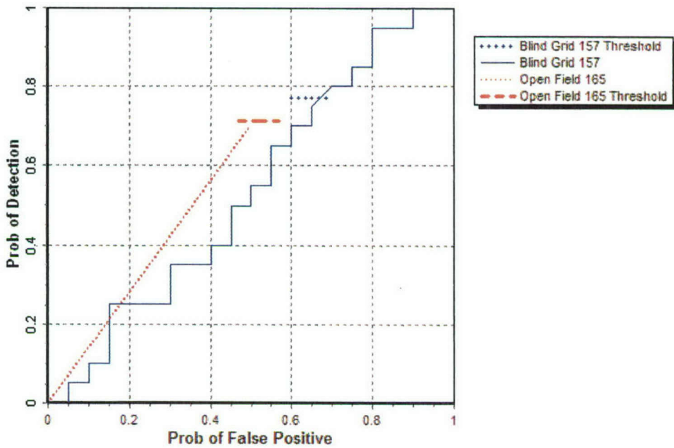
Figure 7. EM61 MKII discrimination stage probability of detection ( P_d^{disc} ) versus the respective probability of false positive ( P_{fp} ) over all ordnance categories combined.
