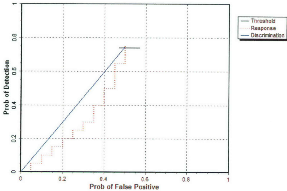
Figure 4. EM61 MKII open field probability of detection for the response stage ( P_d^{\text{res}} ) and the discrimination stage ( P_d^{\text{disc}} ) versus their respective probability of false positive ( P_{fp} ) for all ordnance larger than 20 mm.
