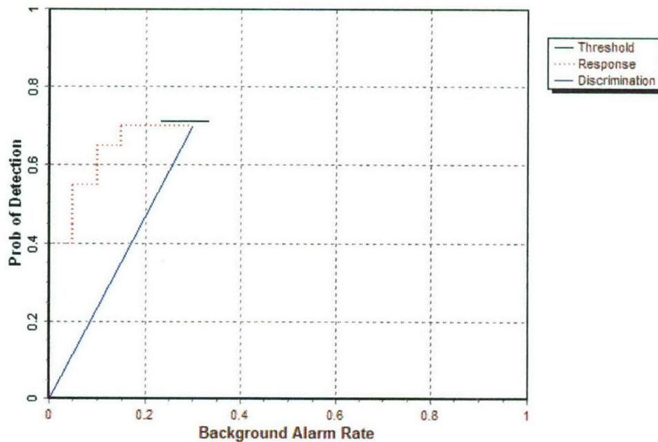
Figure 3. EM61 MKII open field probability of detection for the response stage ( P_d^{\text{res}} ) and the discrimination stage ( P_d^{\text{disc}} ) versus their respective background alarm (BAR) over all ordnance categories combined.
