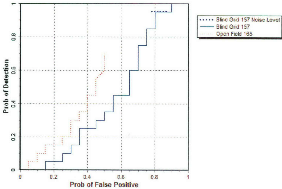
Figure 6. EM61 MKII the probability of detection response ( P_d^{res} ) stages versus the respective probability of false positive ( P_{fp} ) over all ordnance categories combined.
