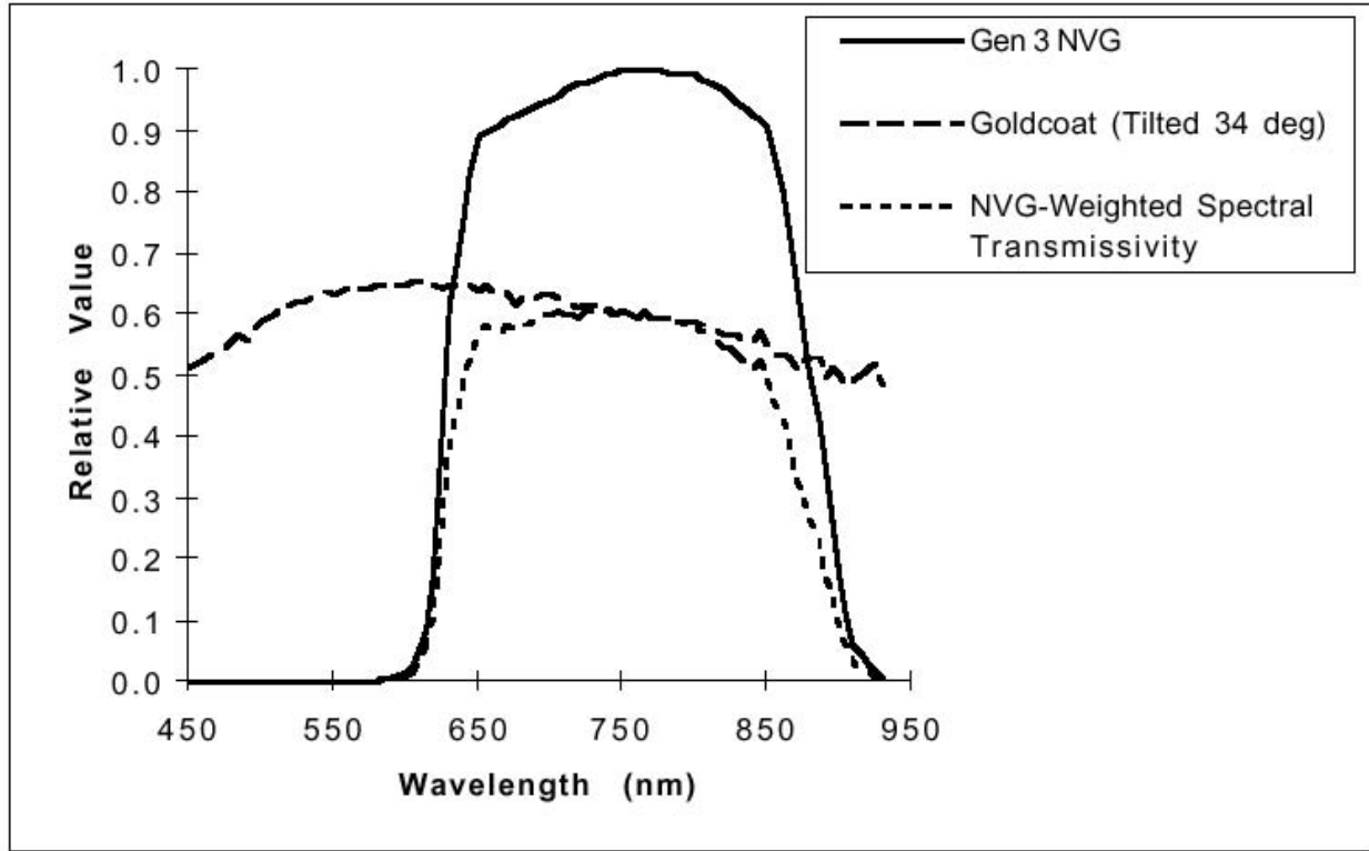
Figure 1. The relative value of a third-generation NVG, a gold-coated transparent sample (34 deg tilt) and its corresponding NVG-weighted spectral transmissivity plotted as a function of wavelength.
