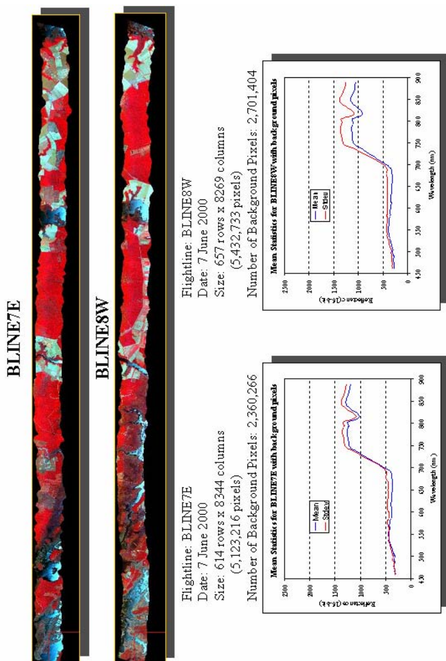
Figure 20. Flightlines BLINE7E and BLINE8W and their associated mean reflectance spectra, including background pixels.
