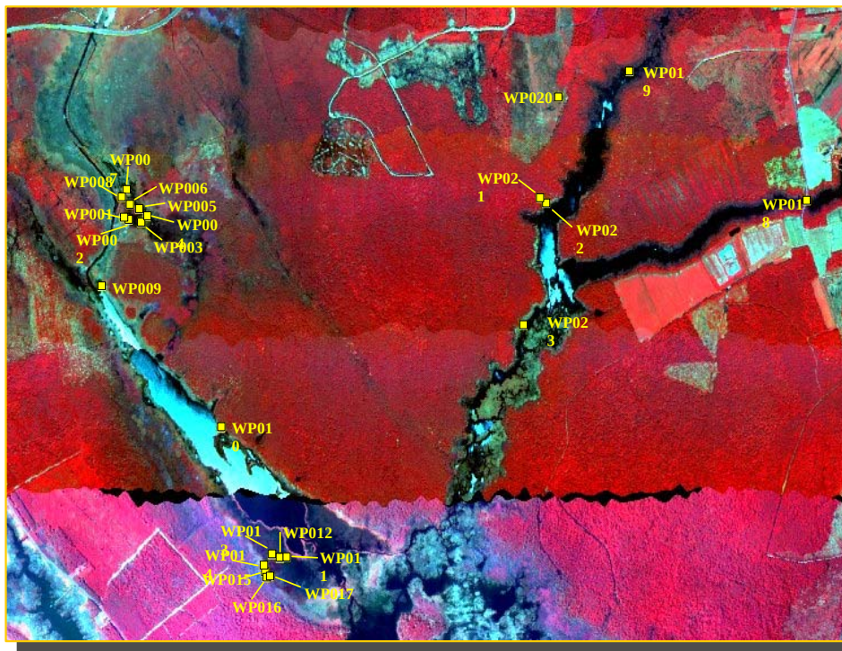
Figure 28. Location of training sites within western part of northern mosaic.
