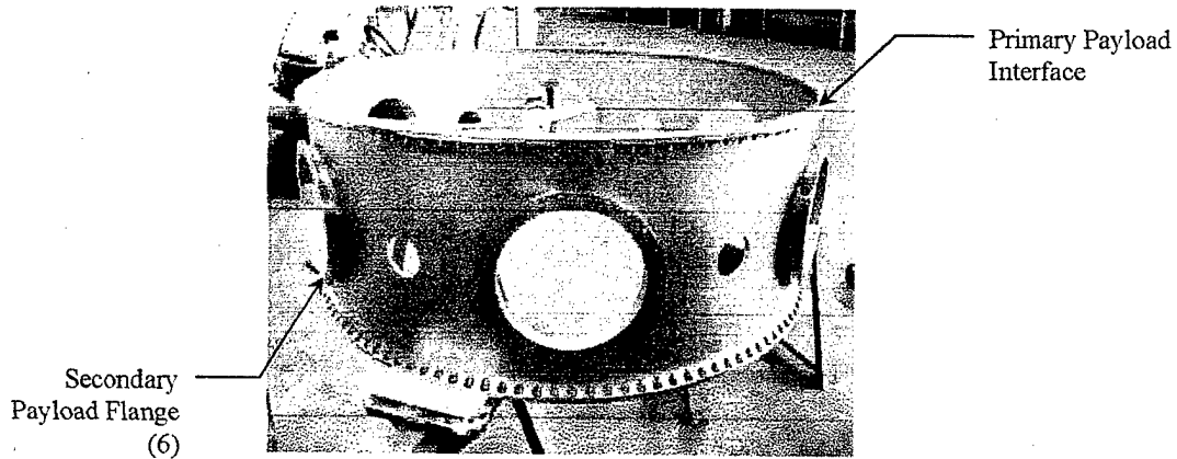
Figure 4. EELV Secondary Payload Adapter (ESPA).
