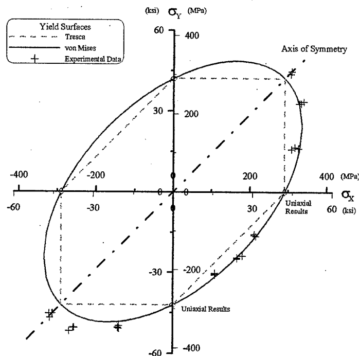
Figure 4. Biaxial Failure Envelope for 6061-T6 Aluminum.
