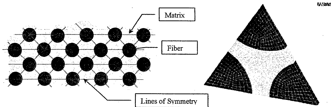
Figure 7. Idealized Lamina Microstructure for the Two Constituent Model and FEA Representative Volume Element (RVE).
