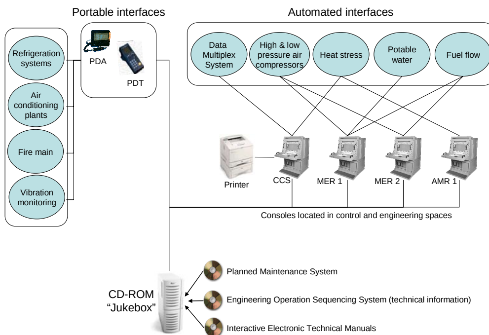
Figure 3. Current Shipboard ICAS Installation
