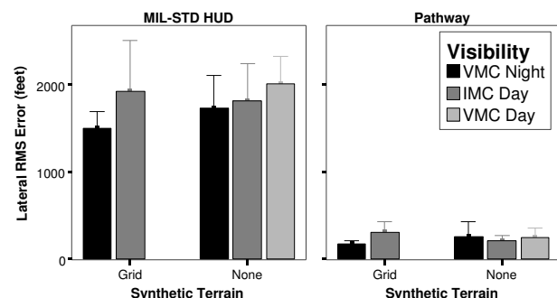
Figure 7. Effects of primary flight display, visibility, and synthetic terrain on Lateral RMSE.
