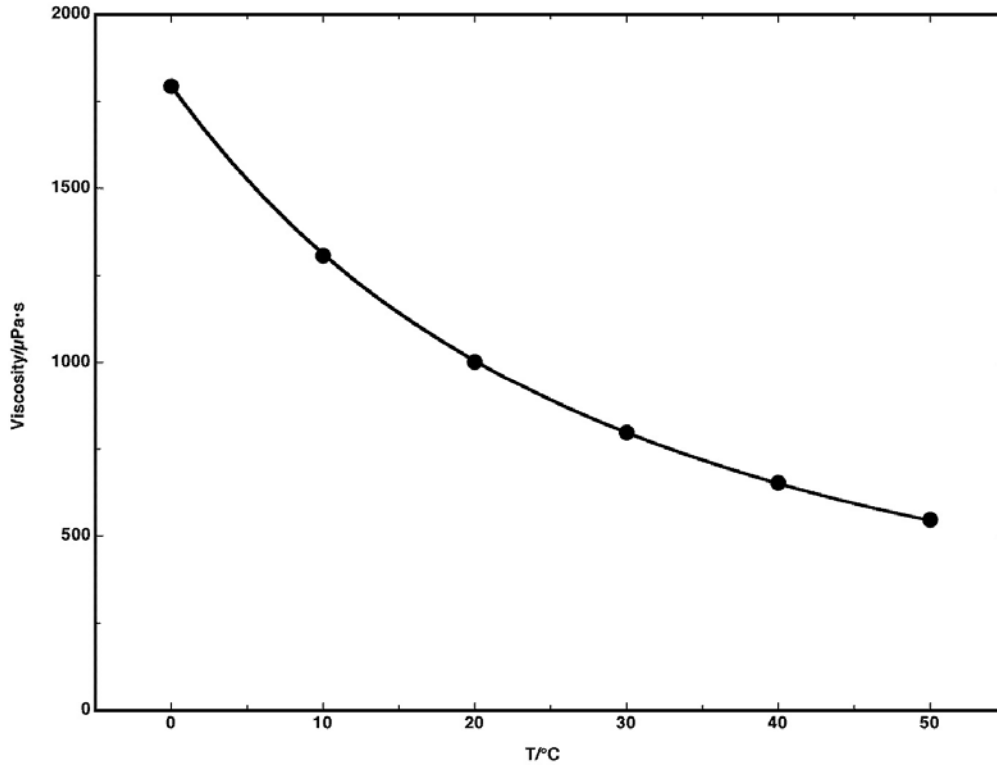
Figure 2. Viscosity of water between 0 and 50 °C.
