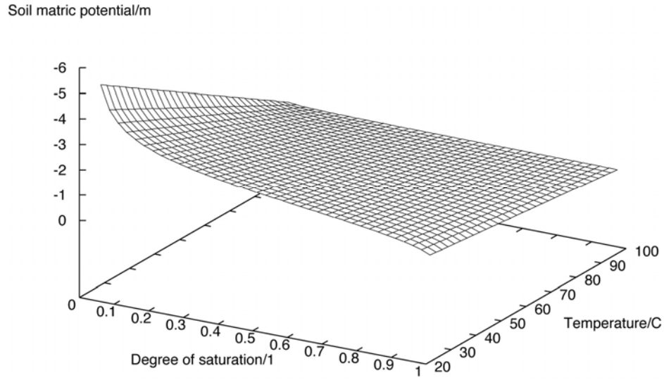
Figure 3. Soil hydraulic head as function of degree of saturation and temperature.
