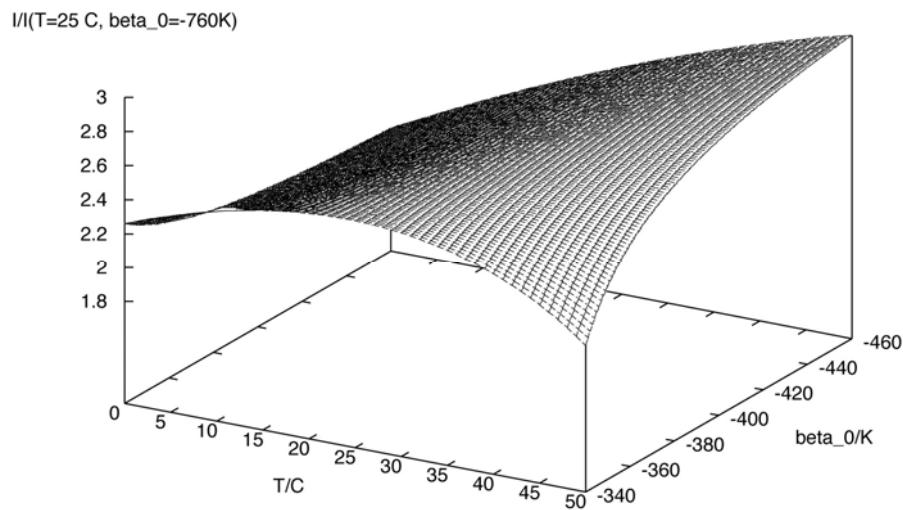
Figure 5. Normalized infiltration as a function of temperature and \beta_0 parameter value.
