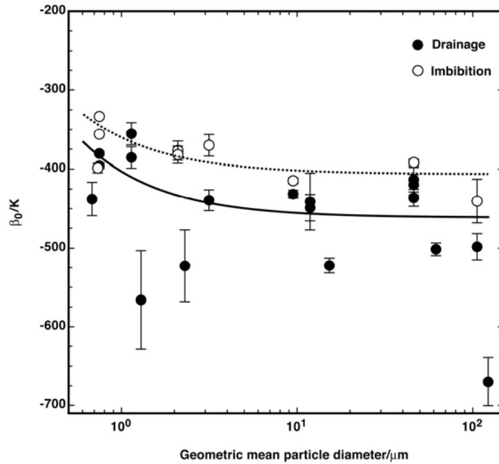
Figure 4. Relationship between \beta_0 parameter and average particle diameter.
