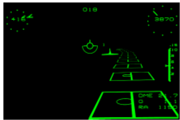
Figure 6. Pathway symbology without HUD STI.
