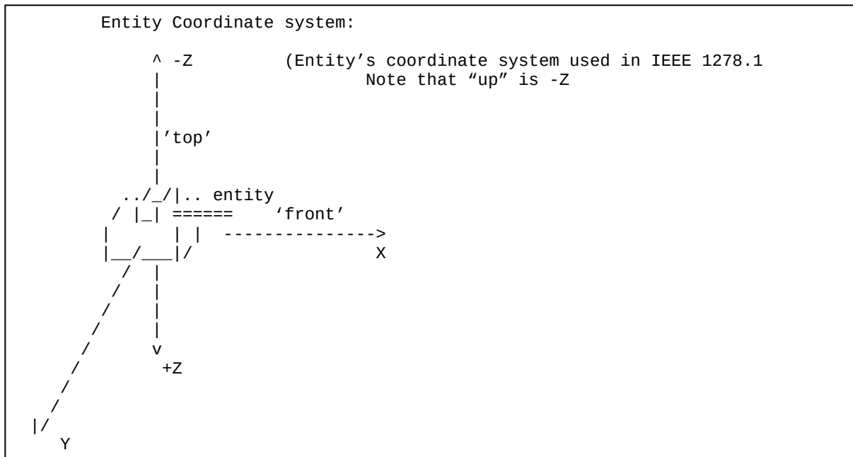
Figure C-3. DIS (IEEE 1278.1) entity coordinate system (ES).
