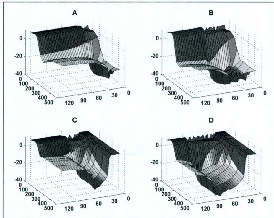
Figure 4. Excess attenuation calculated for sound propagation over discontinuous snow covers of various dimensions. For each plot, the axis on the left is the frequency (Hz) while the axis on the right is the distance (m). The snow cover was located between -30 m and 30 m (A), -30 m and 60 m (B), +30 m and 60 m (C), and 30 m and 90 m (D).
