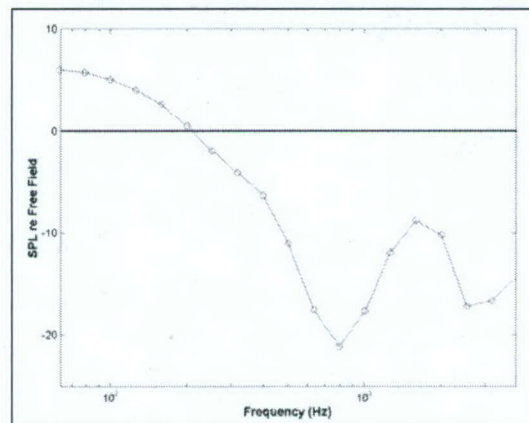
b. Results of the current Open BEM code for the same situation.
