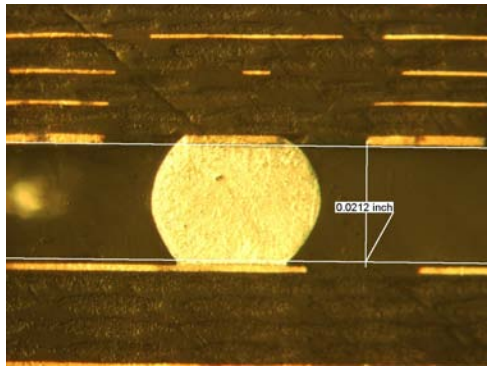
Galileo 388: 0.0212" @ corner
