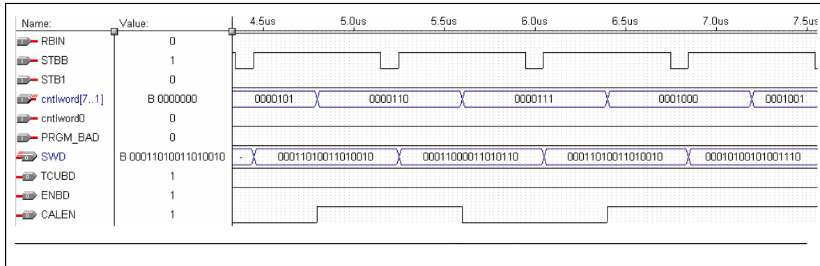
FIGURE 7.11 - Waveform of extracted Truth Table element from VHDL
