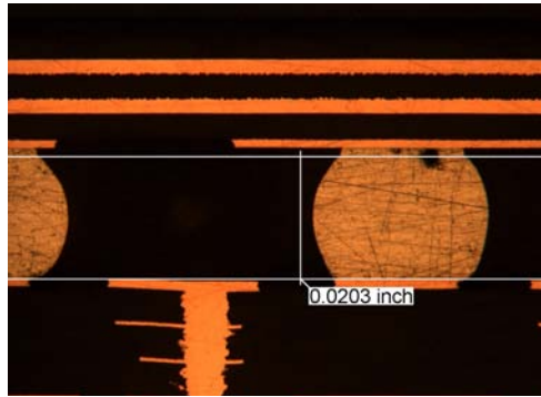
Lattice 388: 0.0203" @ corner
