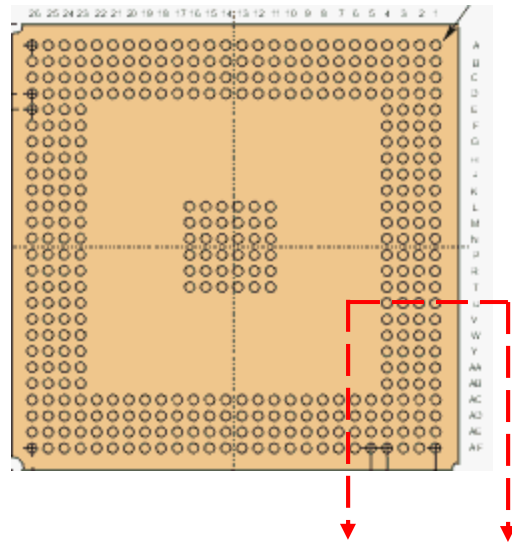
Figure 8.53 - 388 PBGA daisy chain part sectioning plane
