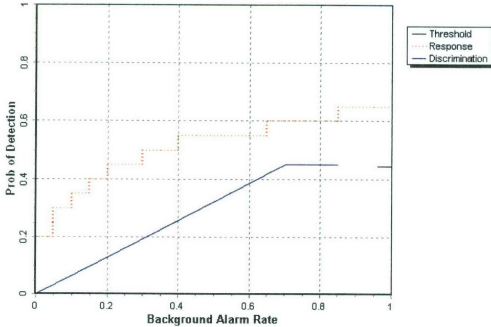
Figure 3. TM-5 EMU open field P_d^{res} and P_d^{disc} versus their respective BAR over all ordnance categories combined.
