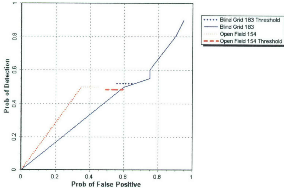
Figure 9. TM-5 EMU P_d^{\text{disc}} versus the respective P_{\text{fp}} for ordnance larger than 20 mm.
