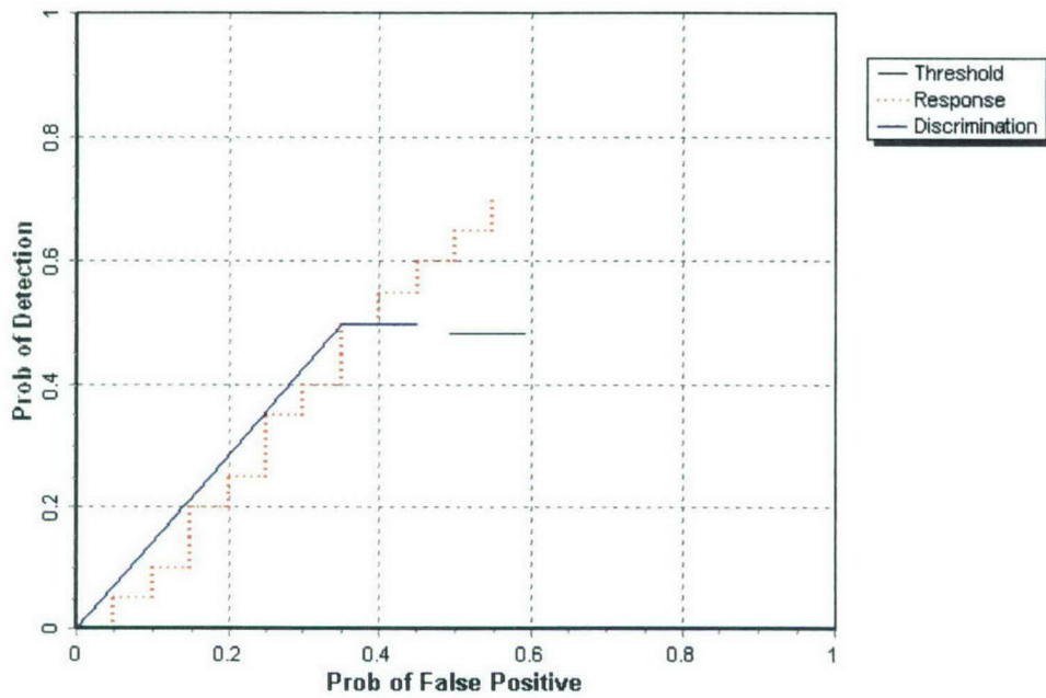
Figure 4. TM-5 EMU open field P_d^{\text{res}} and P_d^{\text{disc}} versus their respective P_{\text{fp}} for all ordnance larger than 20 mm.
