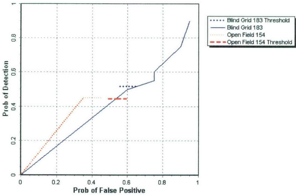
Figure 7. TM-5 EMU P_d^{disc} versus the respective P_{fp} over all ordnance categories combined.
