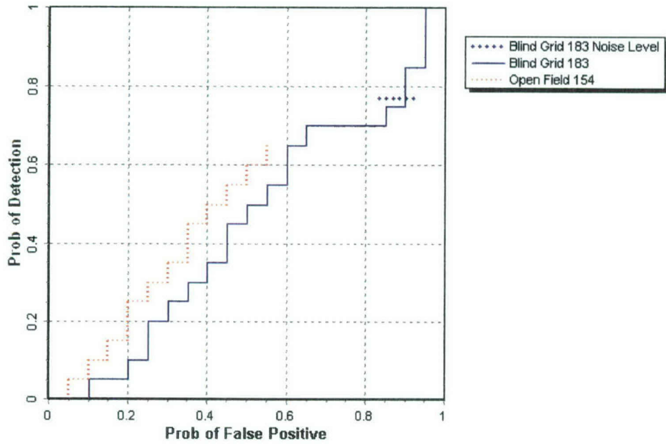
Figure 6. TM-5 EMU P_d^{res} stages versus the respective P_{fp} over all ordnance categories combined.
