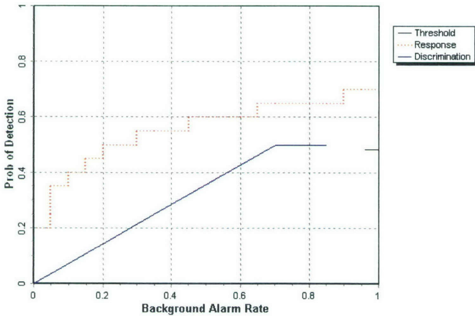
Figure 5. TM-5 EMU open field P_d^{\text{res}} and P_d^{\text{disc}} versus their respective \text{BAR}^{\text{res}} for all ordnance larger than 20 mm.
