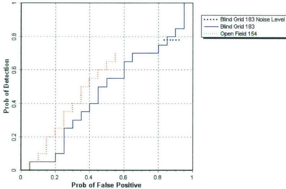
Figure 8. TM-5 EMU P_d^{\text{res}} versus the respective P_{\text{fp}} for ordnance larger than 20 mm.
