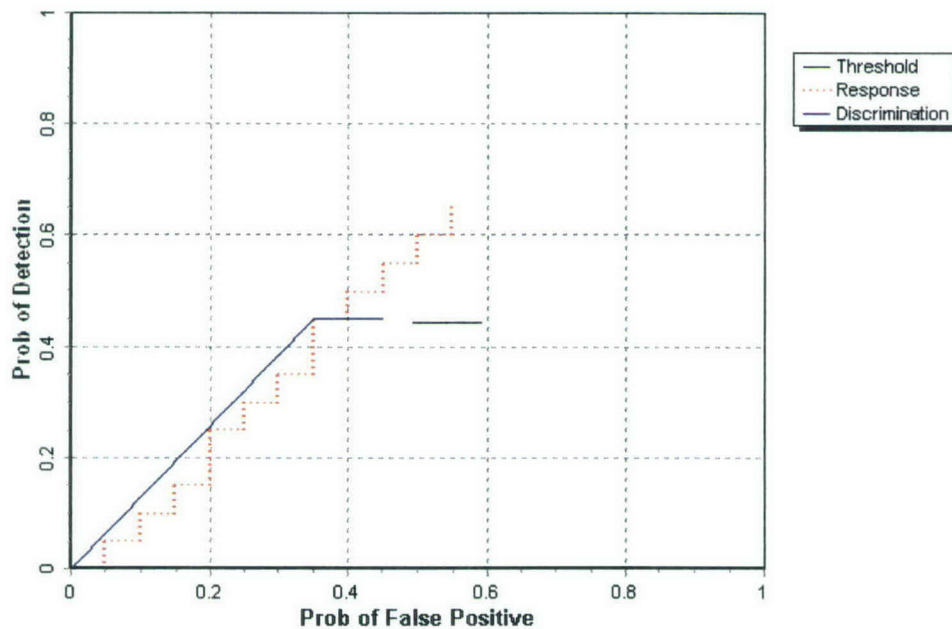
Figure 2. TM-5 EMU open field P_d^{\text{res}} and P_d^{\text{disc}} versus their respective over all ordnance categories combined.
