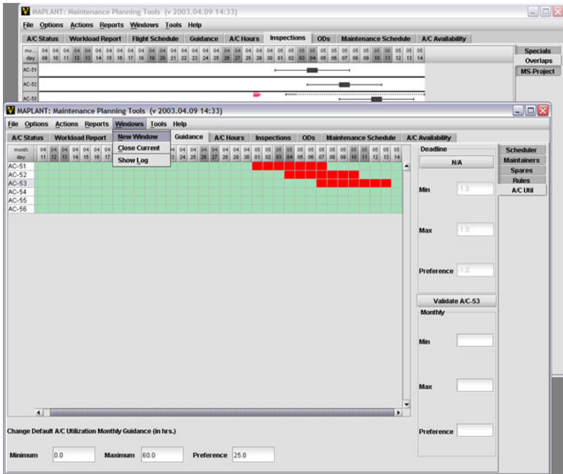
Figure 24. The Windows Menu
