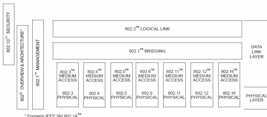
Figure 1. 802.16's Place in the IEEE 802 Standards Hierarchy. (From [2]).
