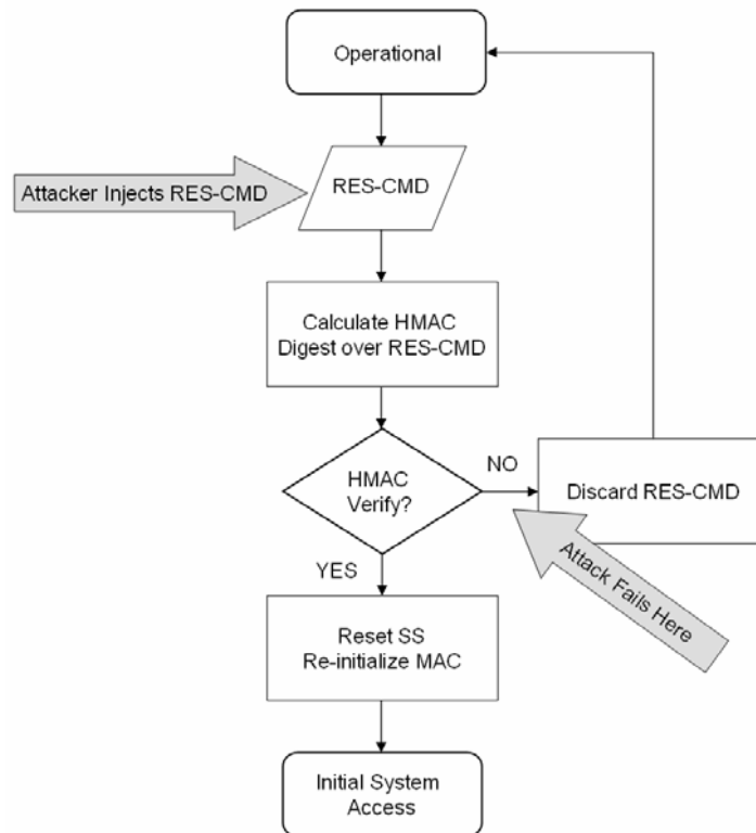
Figure 8. Failure of the Deauthentication Attack using RES-CMD.
