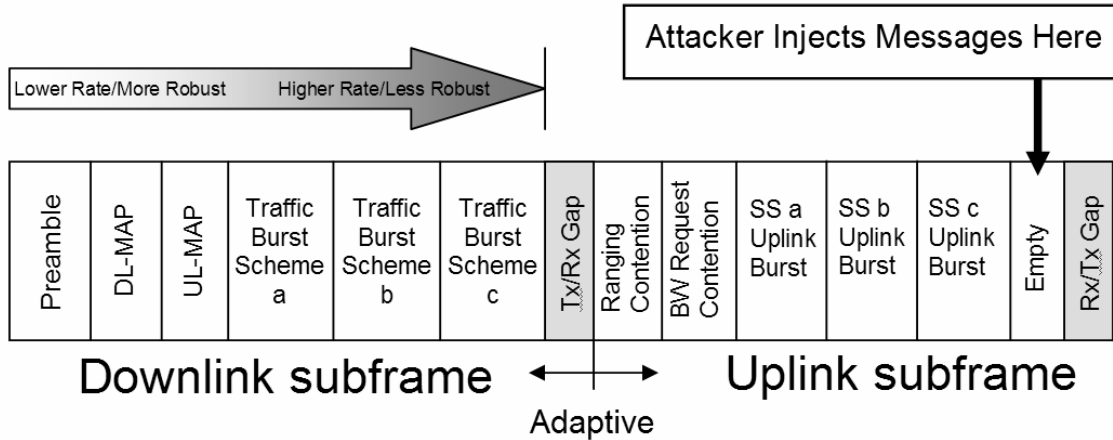
Figure 12. Injecting a Message into a TDD frame. (Synthesized From [2] and [7]).
