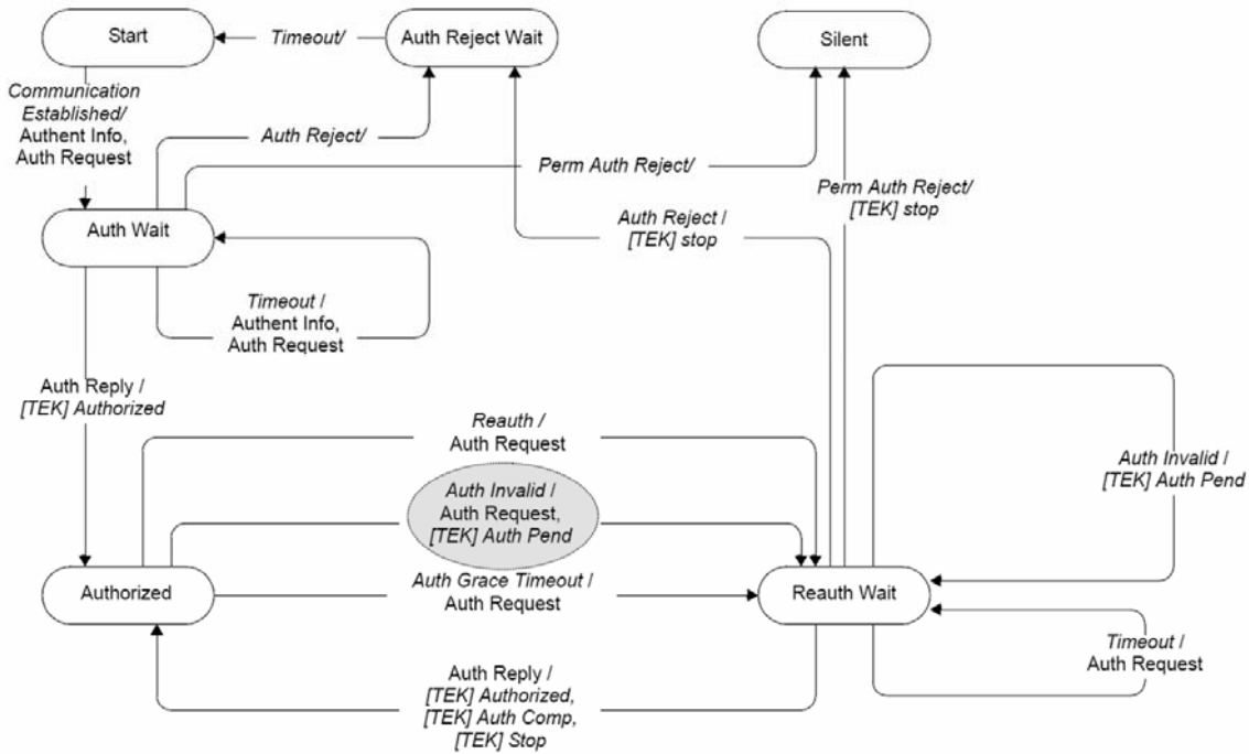
Figure 16. Authorization State Machine Highlighting the Auth Invalid message. (After [3]).
