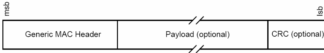
Figure 4. The Format of MAC Management Protocol Data Units. (From [2])
