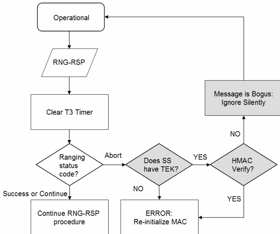
Figure 17. Modified Section of RNG-RSP State Machine. (After [7]).
