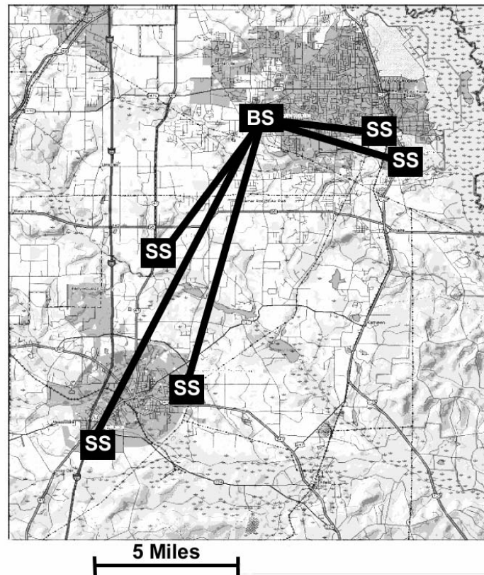
Figure 7. Houston County Test Network. (After [9]).
