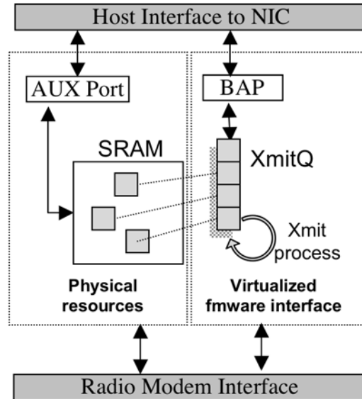
Figure 9. Block Diagram Showing How the AUX Port is used to Circumvent Firmware. (From [12]).
