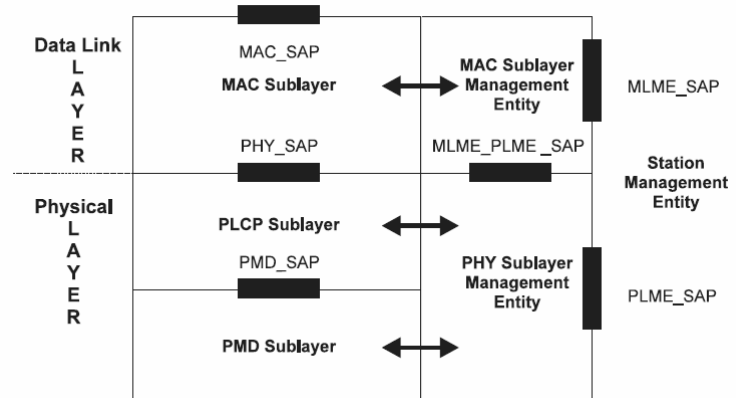
Figure 10. Protocol Layering in IEEE 802.11. (From [11]).
