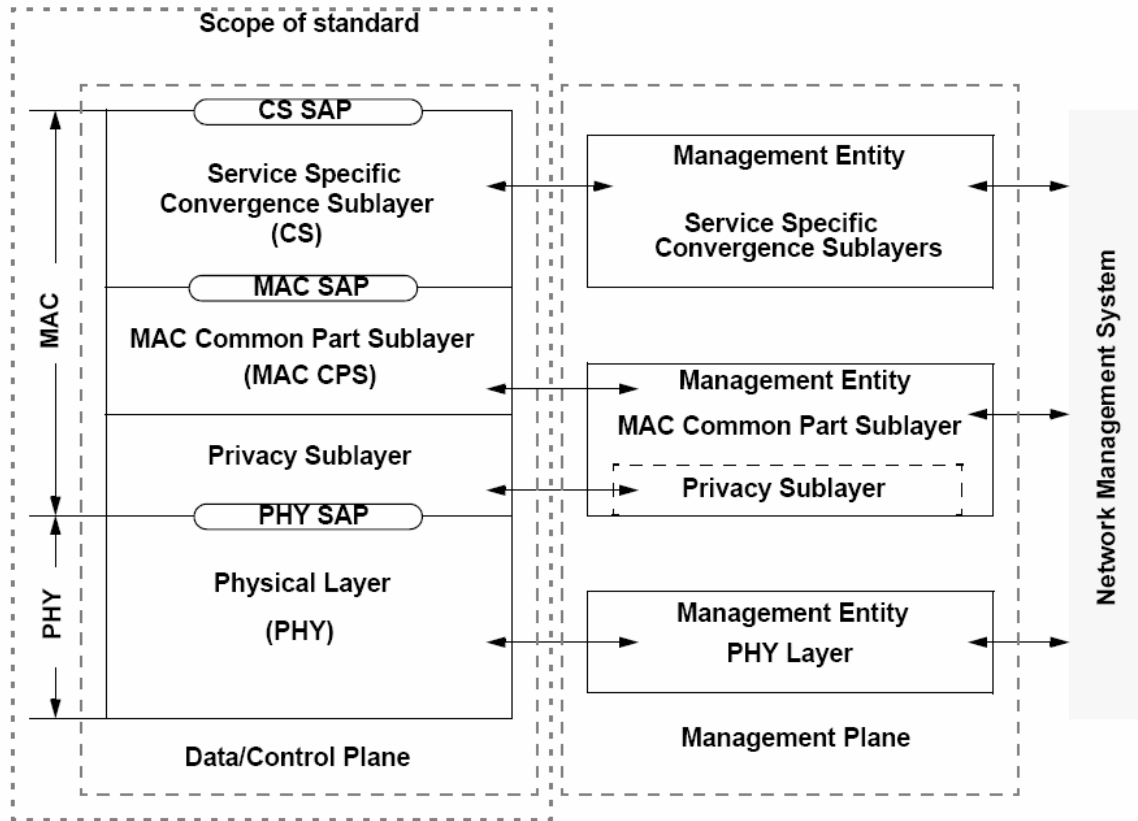
Figure 2. Protocol Layering in IEEE 802.16. (From [2]).
