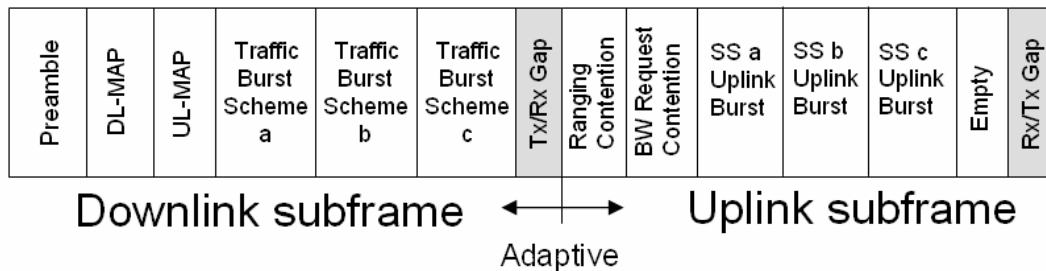
Figure 3. Example of a TDD frame. (Synthesized from [2] and [7]).
