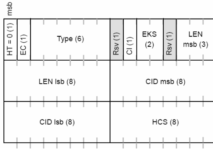
Figure 5. Generic MAC Header Format. (From [3]).
