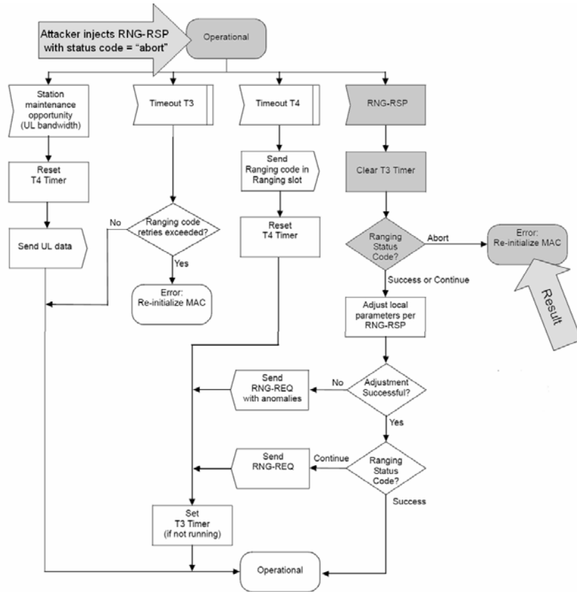
Figure 15. Flow of the RNG-RSP Attack. (After [7]).
