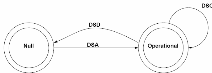
Figure 13. An Overview of the Dynamic Service Flow State Machine. (From [2]).
