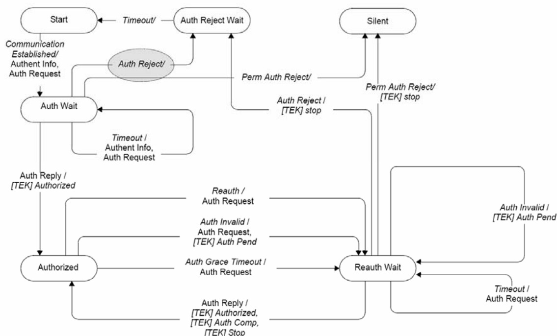
Figure 14. The Authorization State Machine. (From [3]).
