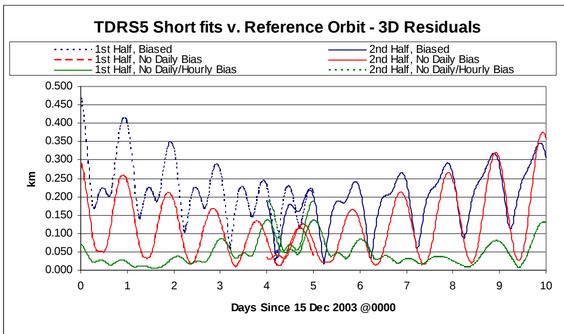
Figure 10 Short TDRS-5 fits compared to reference orbit
