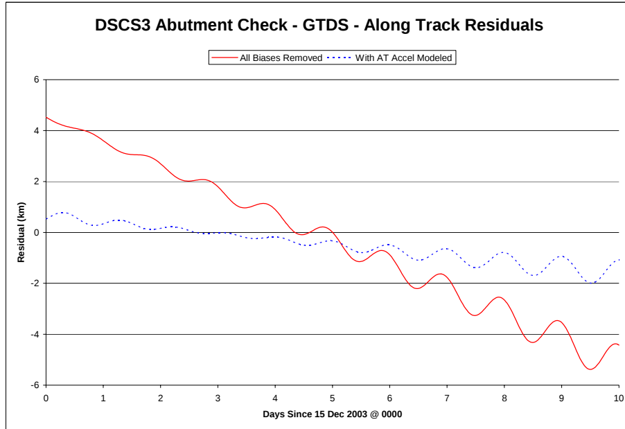
Figure 6 DSCS-3/A1 along-track abutment check with and without acceleration
