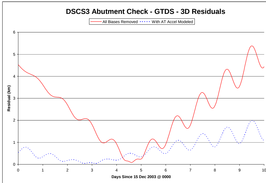
Figure 7 DSCS-3/A1 abutment check with and without acceleration
