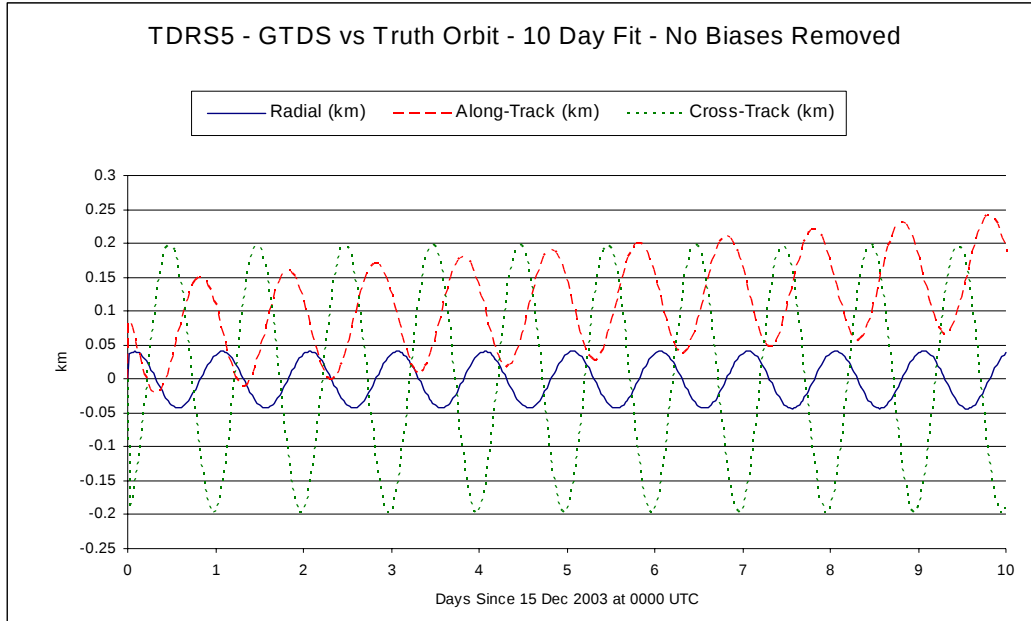
Figure 2 Ten Day Fit Compared to Reference Orbit
