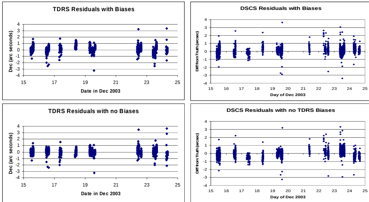
Figure 11 Declination Biases for TDRS-5 and DSCS-3/A1
