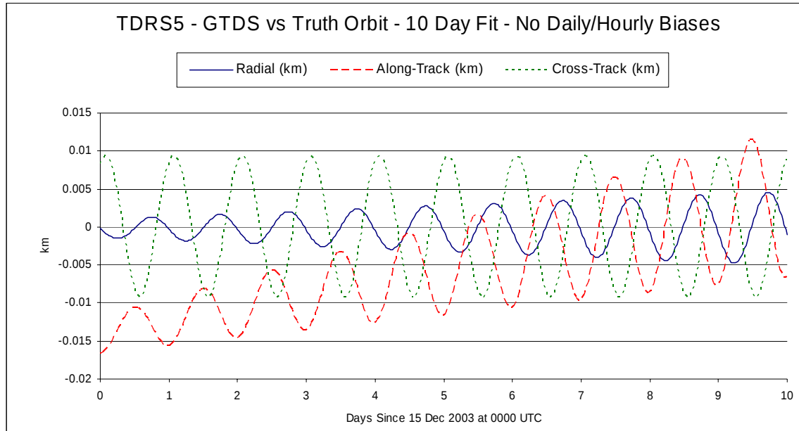
Figure 4 Ten Day Fit Compared to Reference Orbit
