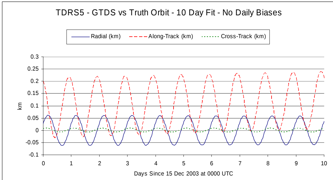
Figure 3 Ten Day Fit Compared to Reference Orbit
