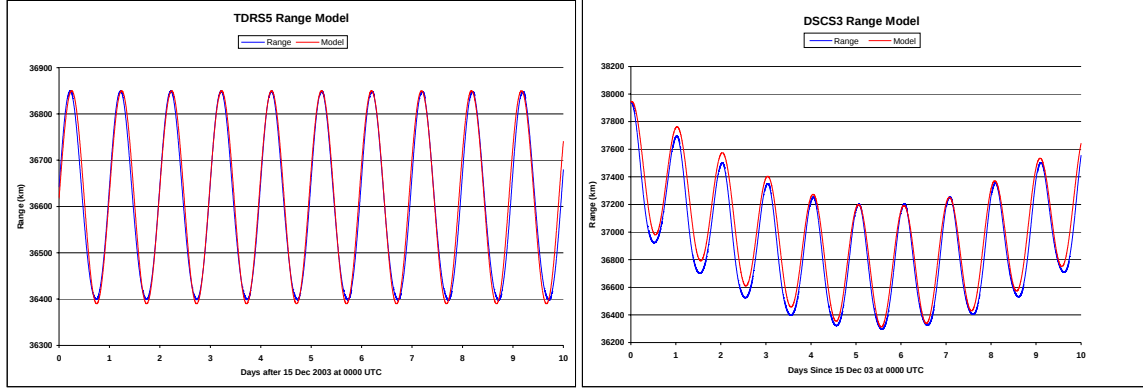
Figure 1 Derived Models for TDRS-5 and DSCS-3 Range, 15-25 Dec 2003
