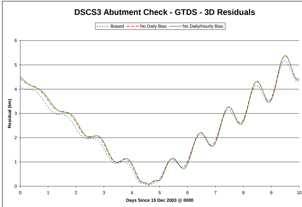
Figure 5 DSCS-3/A1 Abutment Check
