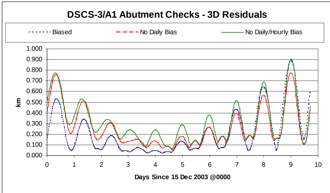
Figure 8 DSCS-3/A1 abutment check with and without TDRSS-based calibration
