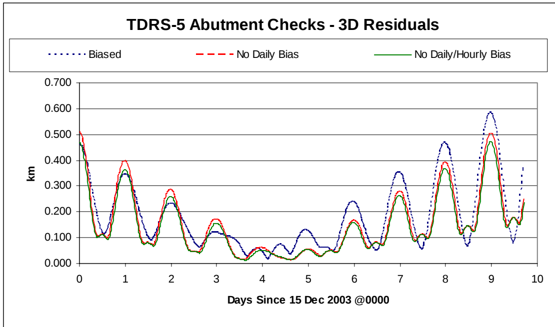
Figure 9 TDRS-5 Abutment Check
