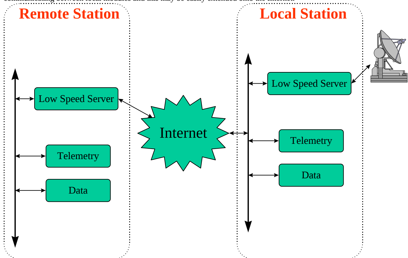
Figure 3. Implementation of spacecraft control over the Internet
