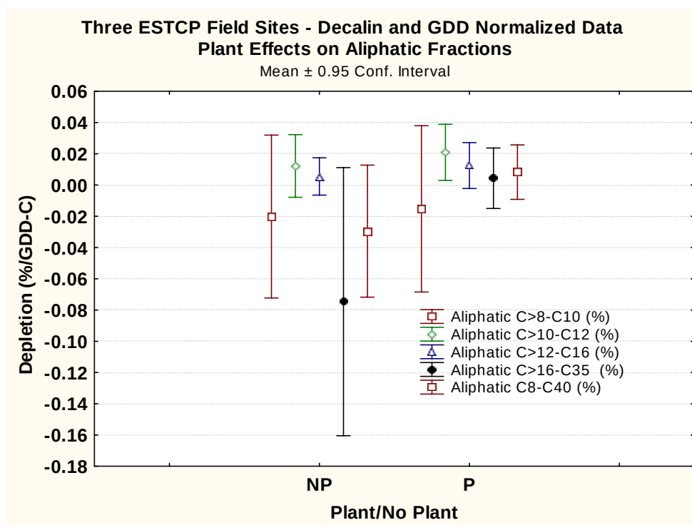
Figure 11. Three ESTCP field sites - decalin and GDD normalized data – plant effects on aliphatic fractions.
