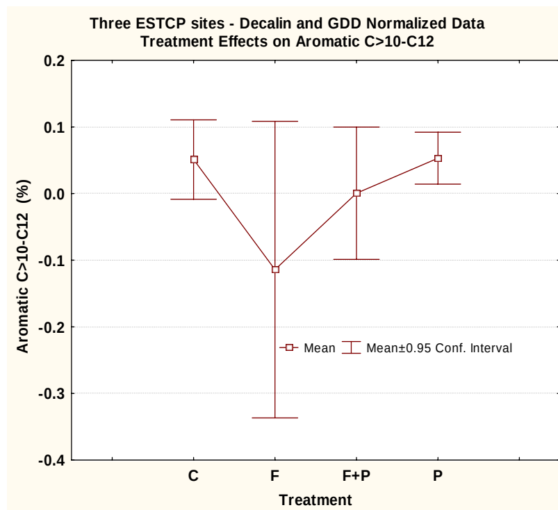
Figure 9. Three ESTCP field sites - decalin and GDD normalized data – treatment effects on aromatic C>10-C12.
