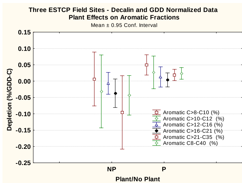
Figure 12. Three ESTCP field sites - decalin and GDD normalized data – plant effects on aromatic fractions.
