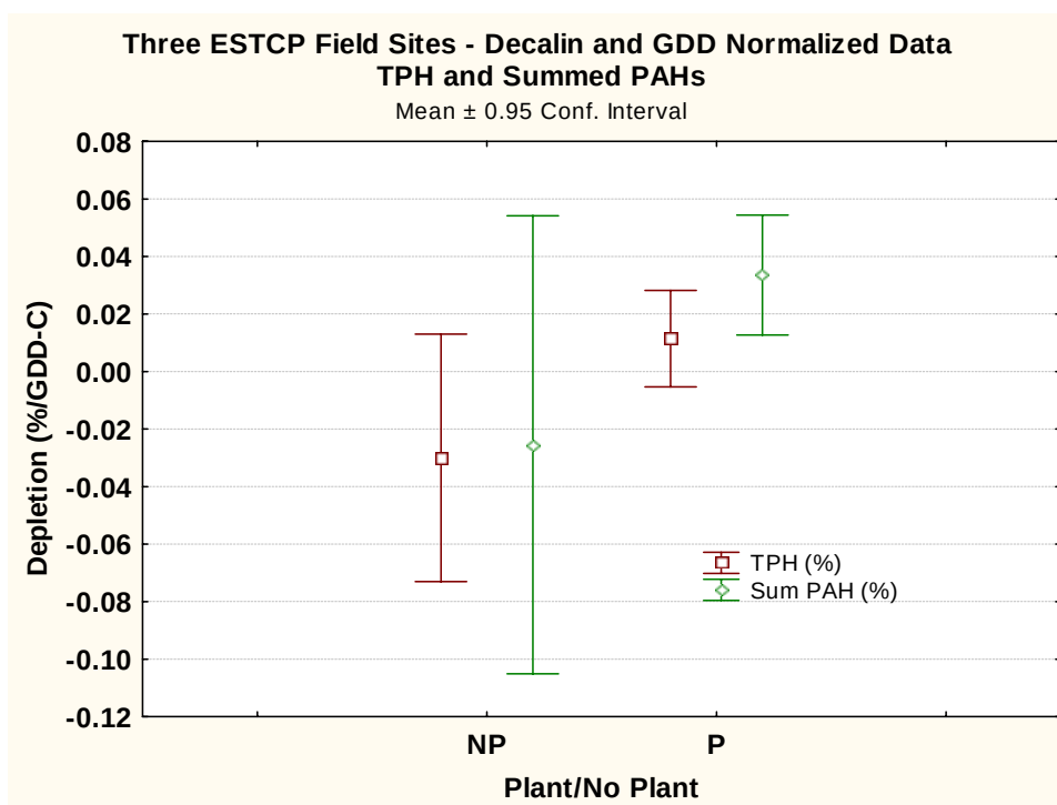
Figure 10. Three ESTCP field sites - decalin and GDD normalized data – plant effects on TPH and summed PAHs.
