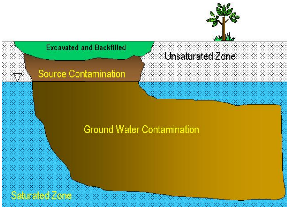
Figure 5. Depiction of soil contamination serving as a source for groundwater contamination.
