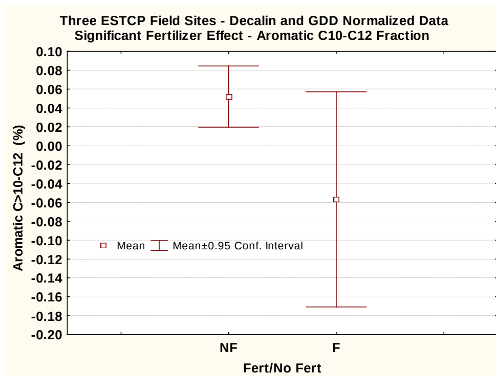
Figure 14. Three ESTCP field sites - decalin and GDD normalized data – significant fertilizer effects (inhibition) on depletion of aromatic C>10-12 fraction.
