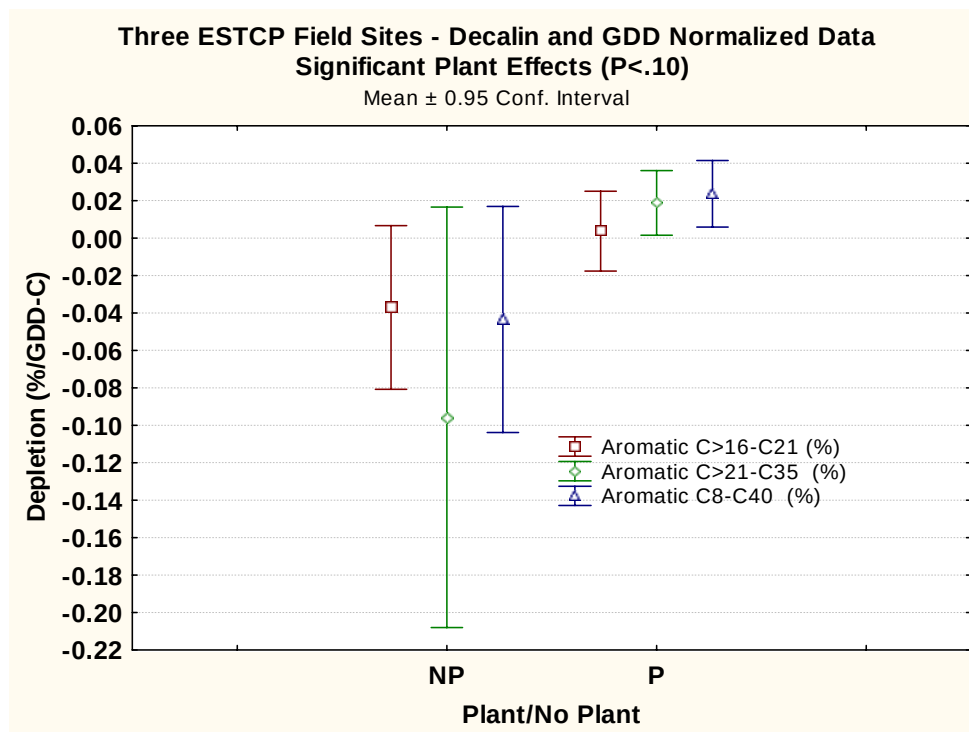
Figure 13. Three ESTCP field sites - decalin and GDD normalized data – significant (P<0.10) plant effects on aromatic fractions.
