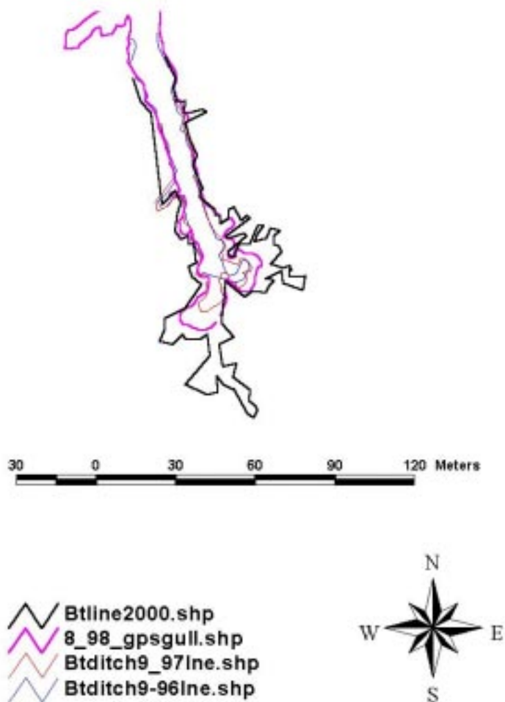
Figure IV-1-2. Monitored erosion of the Bread Truck drainage ditch from 1996 to 2000 showing the edge of the deep gully as monitored by surveying or GPS.
