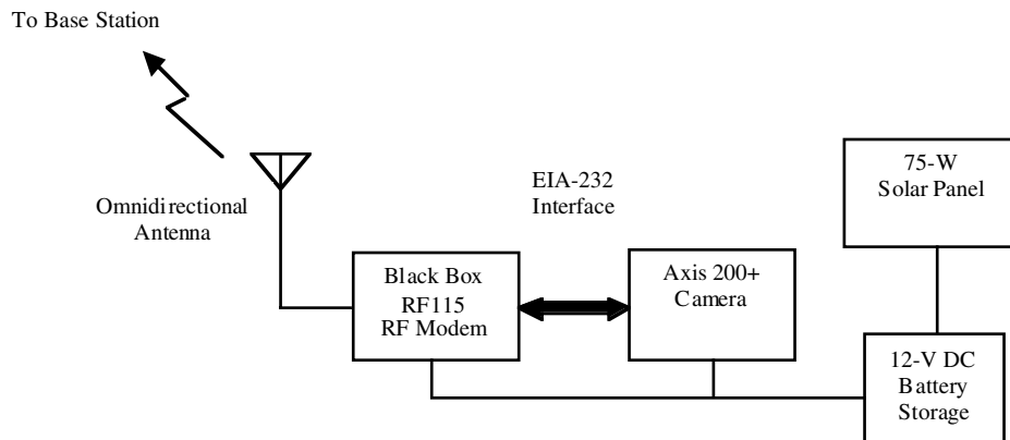
Figure III-5-1. Remote site equipment.
