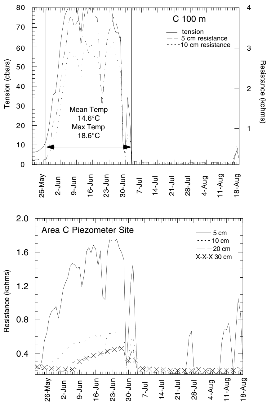
Figure III-2-9. Output from moisture sensors during the summer of 2000. Increases in resistance and tension indicate drying. Temperatures are 24-hour averages. High temperatures increase the rate of loss of white phosphorus.
