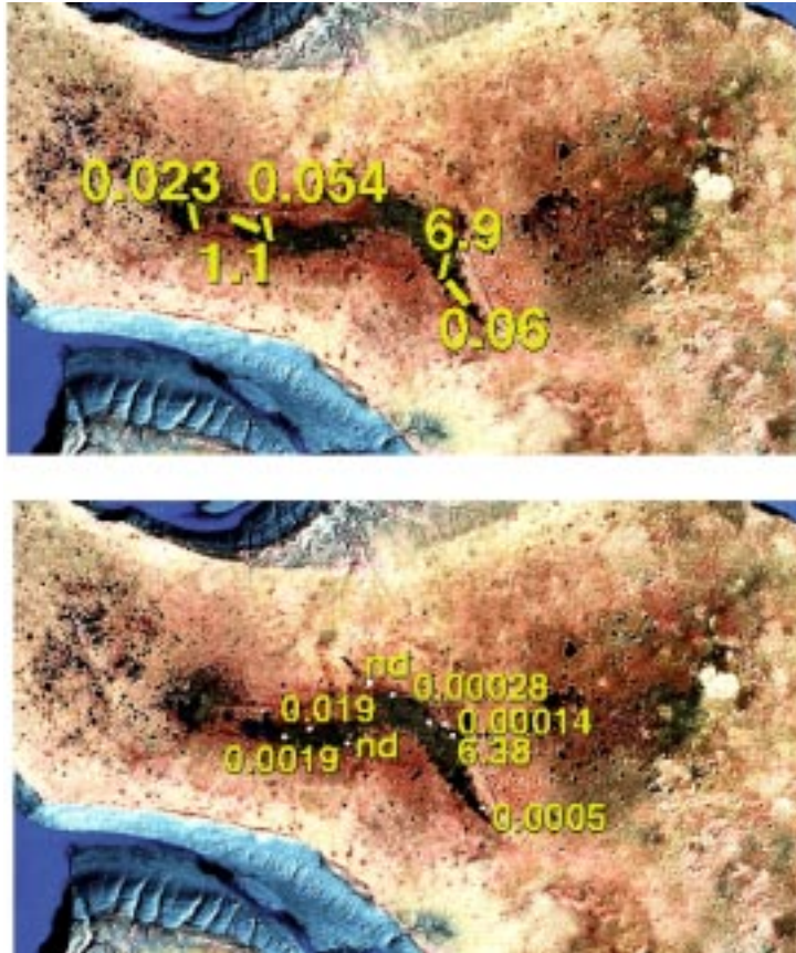
Figure III-2-6. White phosphorus concentrations ( \mu\text{g/g} ) found in composite (top) and discrete (bottom) samples collected August 2000 from the Aquablok-treated pond (#285) on Racine Island (nd = not detected).
