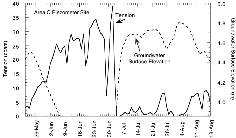
Figure III-2-10. Groundwater surface elevation in the piezometer well located in Area C and the corresponding moisture content (tension) of the surface sediment (elevation 4.77 m). A rise in tension indicates drying.
