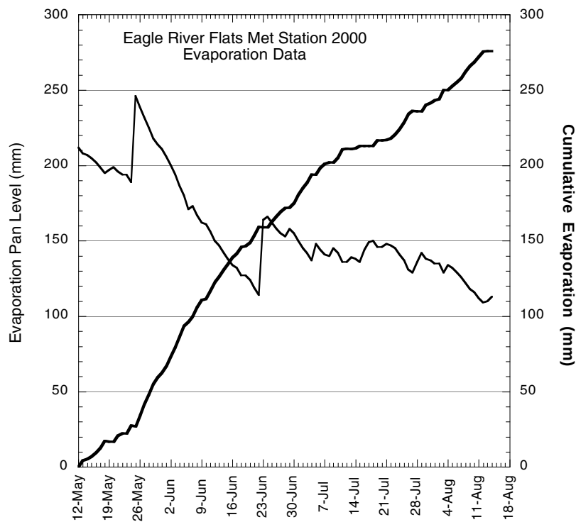
Figure III-4-5. Evaporation pan data showing the evaporation pan water level data and the net cumulative evaporation for the season. The steepness of the net cumulative curve in June reflects the warm temperatures and good drying conditions during this period. The evaporation pan water level data show the decrease in the water level due to evaporation, the addition of make-up water on 25 May and 23 June, and the contribution from periodic rainstorms throughout July.
