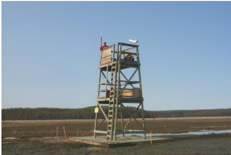
Figure III-5-3. Placement of the remote site equipment in the field.
