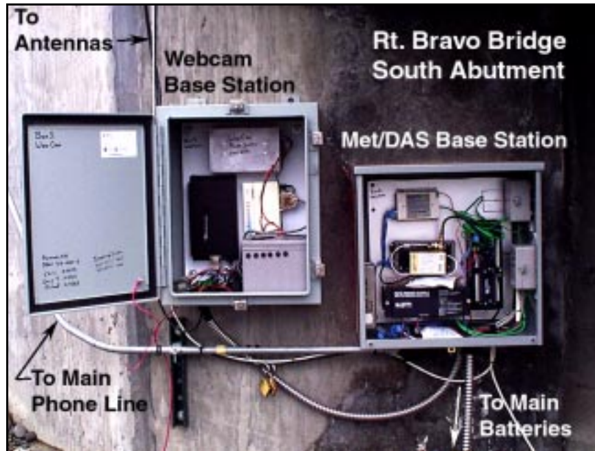
Figure III-1-2. Rt. Bravo Bridge remote monitoring base station.
