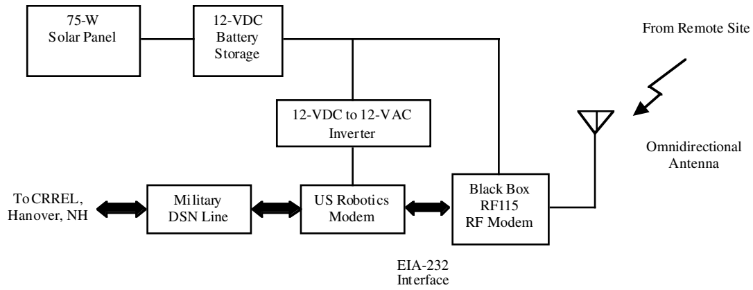
Figure III-5-4. Base station equipment.
