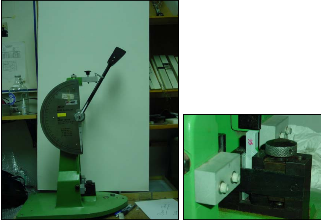
Figure 40. Izod testing machine with the samples shown in the anvil in the inset.
