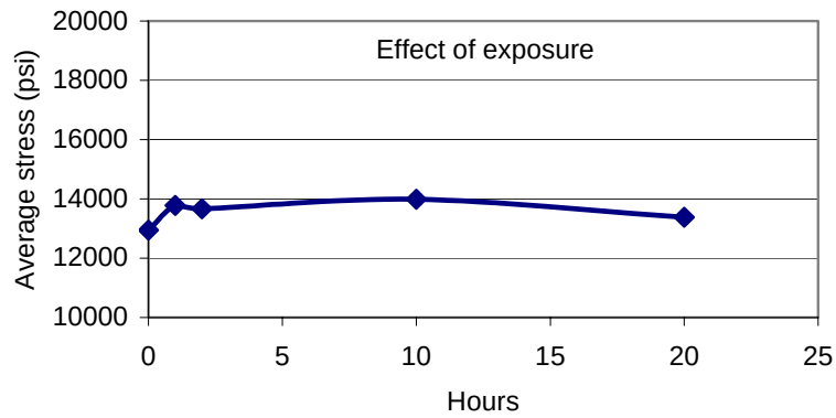
Figure 48. Average values of yield stress after boiling
