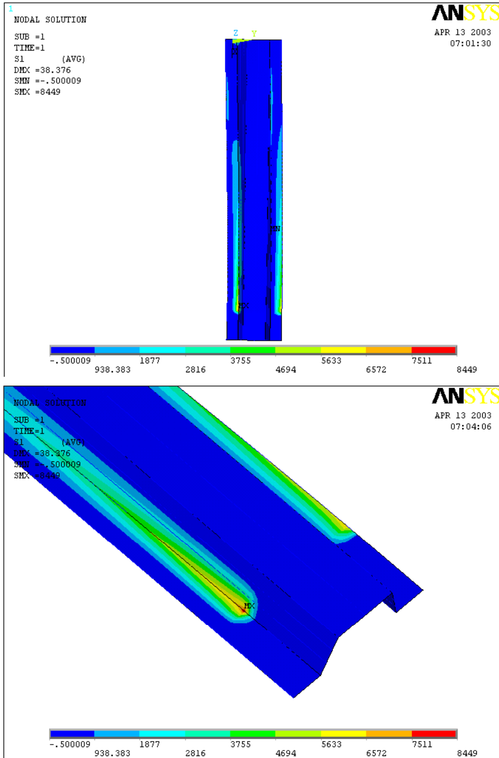
Figure C6. First principal stress distribution in the seawall structure.
