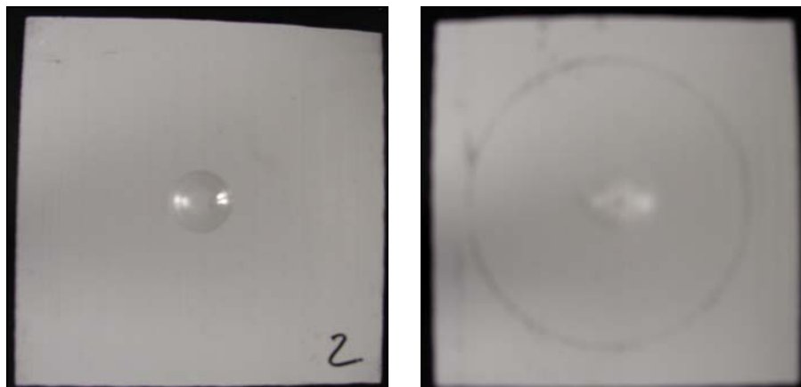
Figure 23. Front and back faces of the low-velocity-impacted PVC control specimen.
