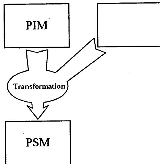
Figure 2: Model Transformation
