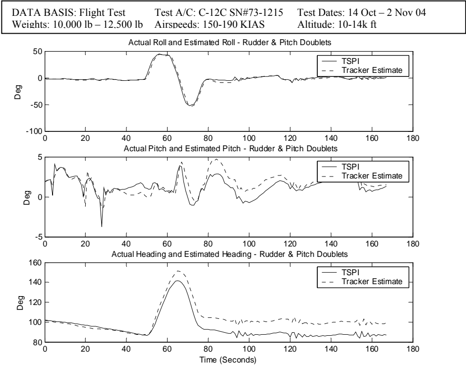
Figure C-17. Head Tracker Angular Performance during Pitch/Rudder Doublets
