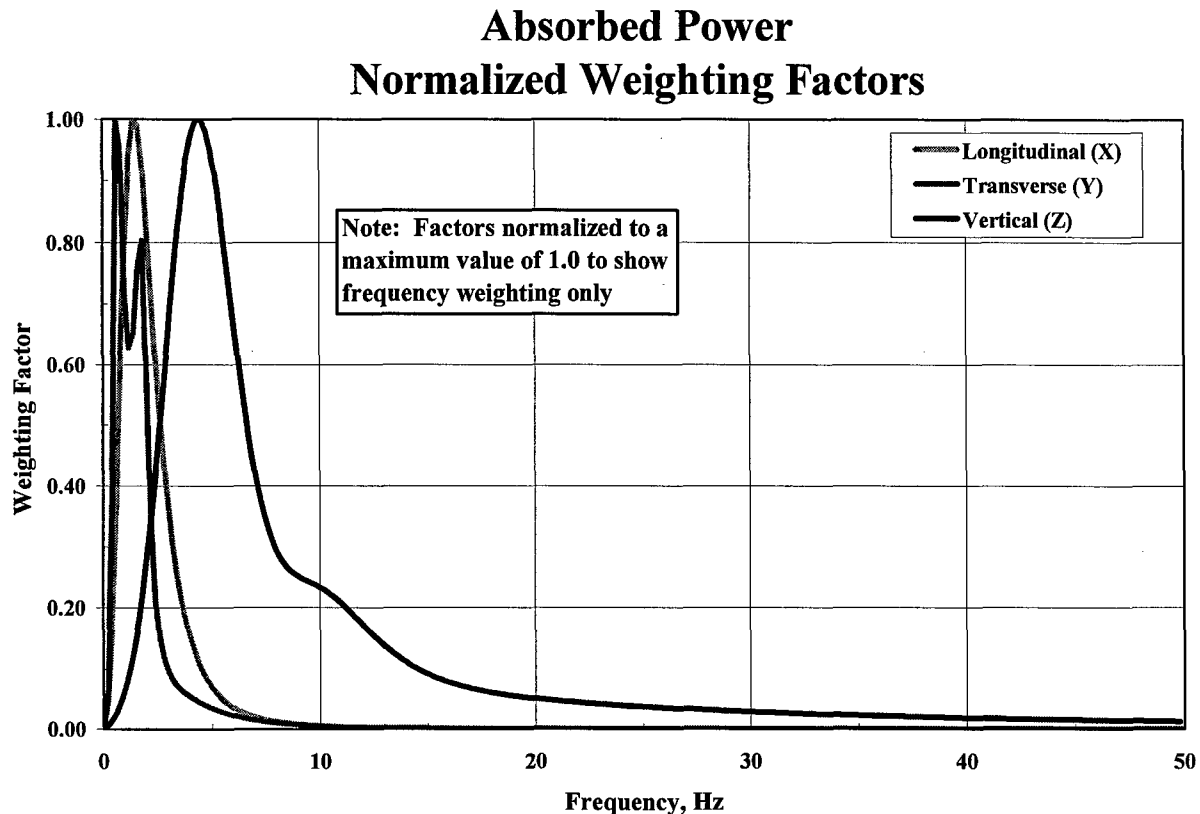
Figure 5. Absorbed Power Normalized Frequency Weighting Factors
