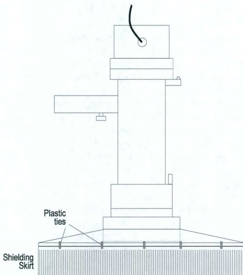
Figure 2. Modified applicator.
