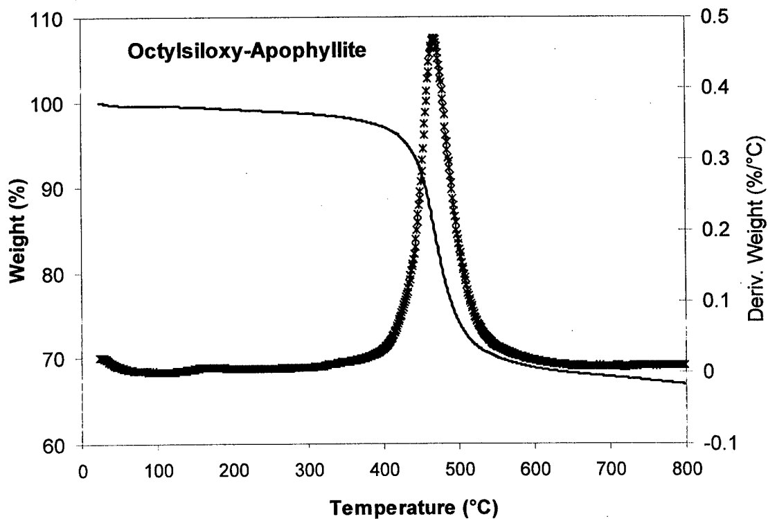
Figure 5. TGA Spectrum of the n -octylsiloxo-Apophyllite under Nitrogen at 2°C/min.
