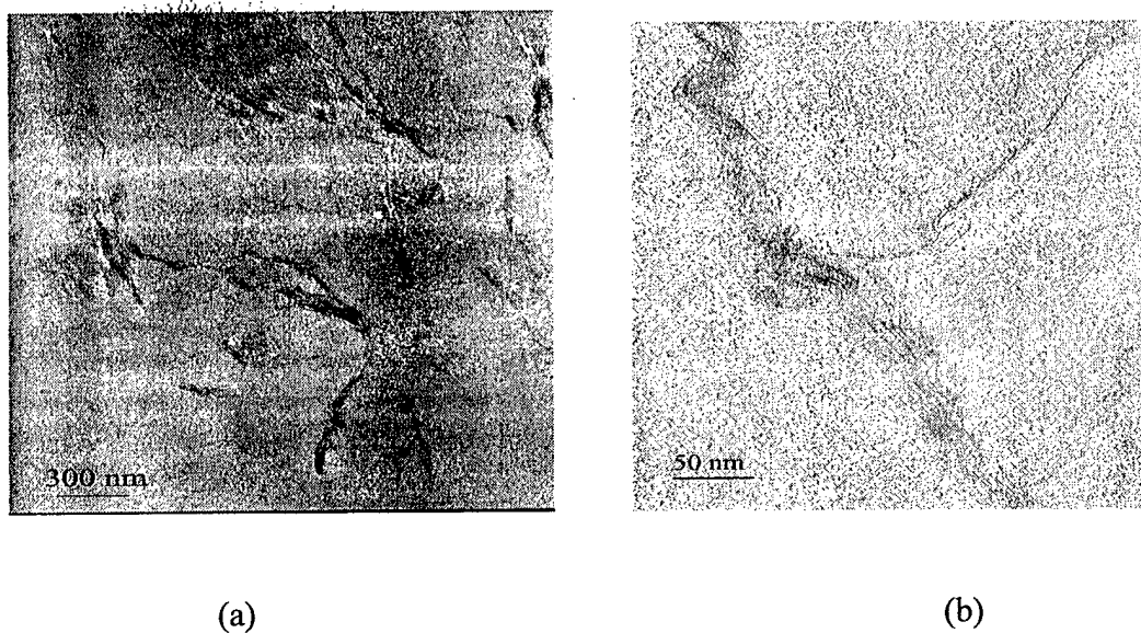
Figure 7. TEM images of vinyl ester nanocomposite. (a) and (b) are the low and high magnification images of 7 octenyl apophyllite clay vinyl ester sample.
