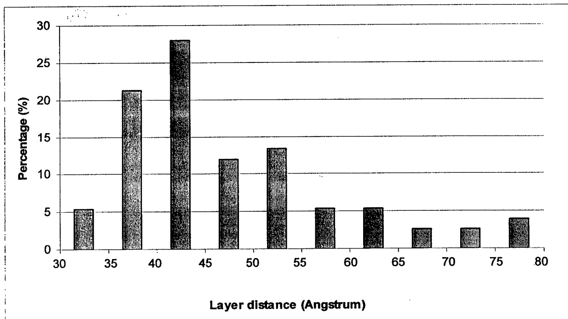
Figure 15 Histogram representation of the distribution of clay platelet separation in a ultrasonication mixed NB-HDMIM-MMT epoxy nanocomposite sample.
