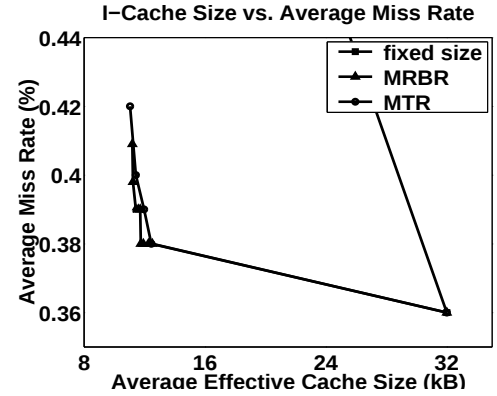
Figure 9: Miss rate versus effective cache size for L1 instruction cache. MTR and MRBR have similar performance.
