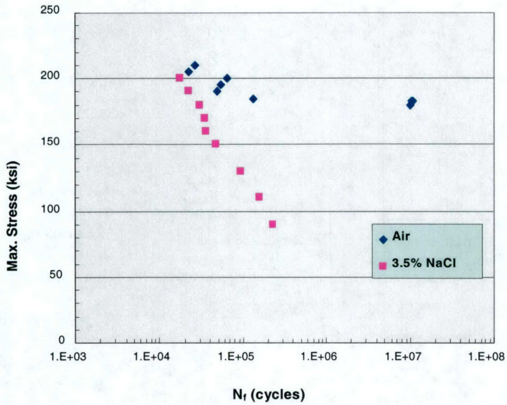
Figure A-5: Stress-Life Curves for Bare Hy-Tuf Steel in Air and 3.5% NaCl Solution
