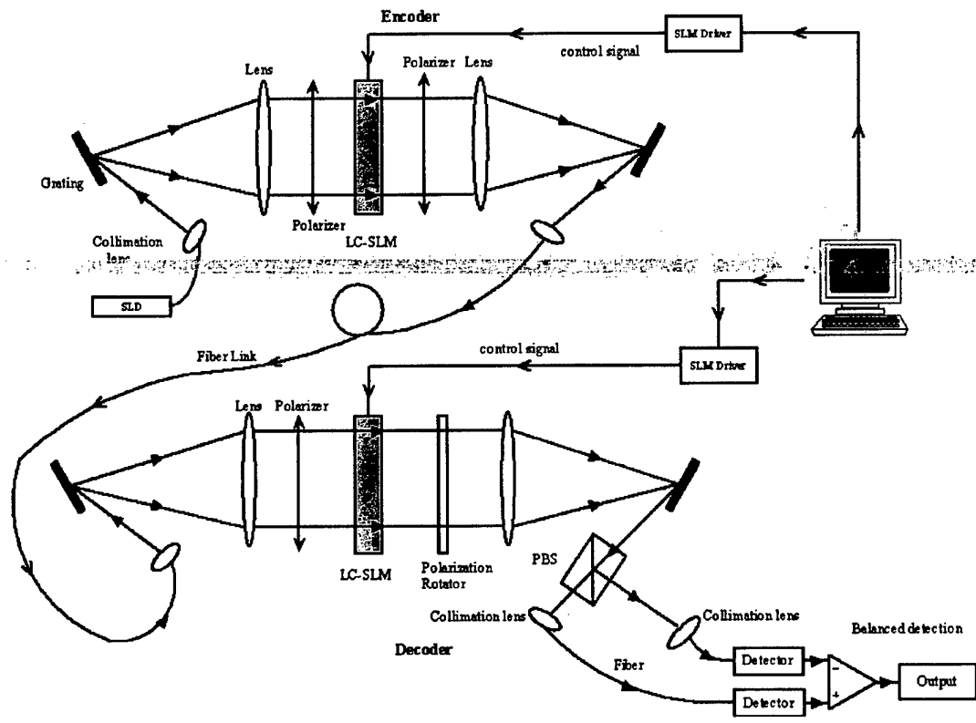
Fig. 3.4: Fiber-based testbed for spectrum encoding and decoding.
