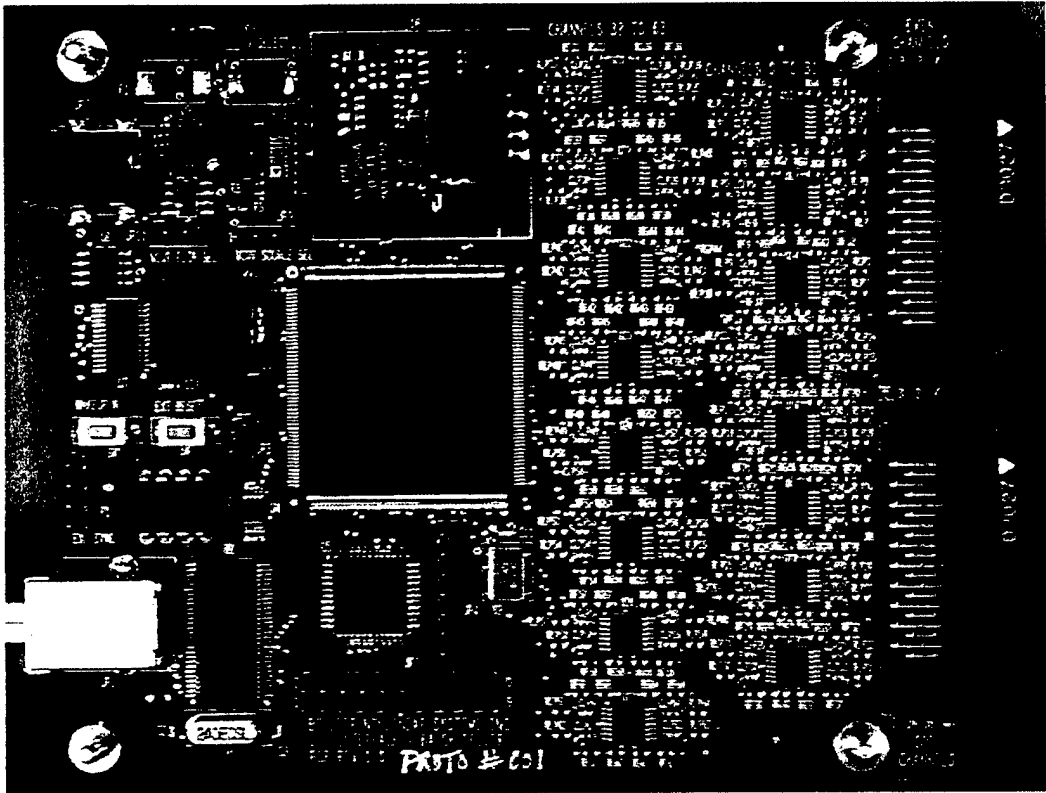
Figure 2.7: A picture of the USB interface – 64 Channel Nematic Driver Board.
