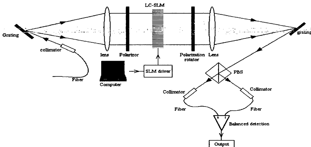
Fig. 3.10(a): Sketch of fiber-based decoder.
