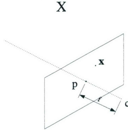
Figure A-1: The pinhole camera. The ray from the scene point \mathbf{X} to the camera center \mathbf{c} intersects the imaging plane at \mathbf{x} . The imaging plane is at a focal length f from the camera center. The projection of the camera center onto the imaging plane is the principal point \mathbf{p} . The ray from \mathbf{c} to \mathbf{p} is the optical axis (dashed).
