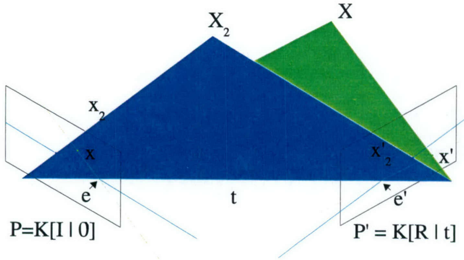
Figure A-3: Multiple epipolar planes intersect on the baseline t and define the epipoles \underline{e} and \underline{e}' on the imaging planes.
