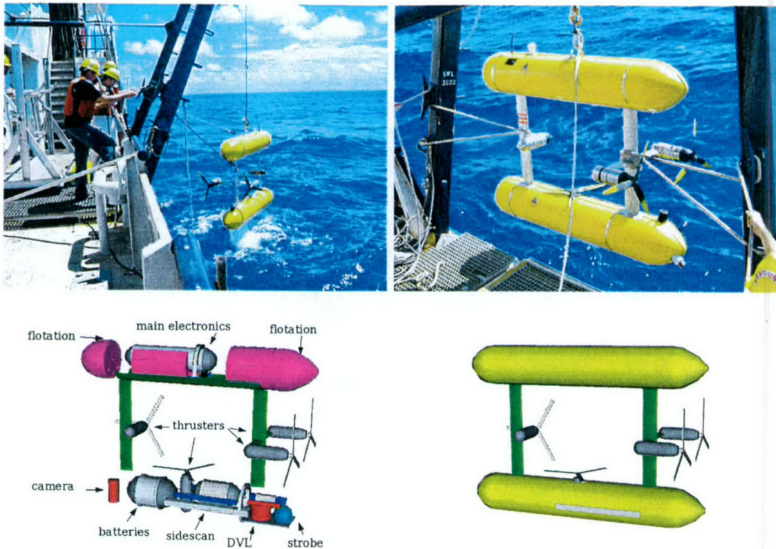
Figure 1-4: (top) The Seabed vehicle in the Bermuda 2002 cruise. (bottom) CAD views showing the vehicle with and without shells.
