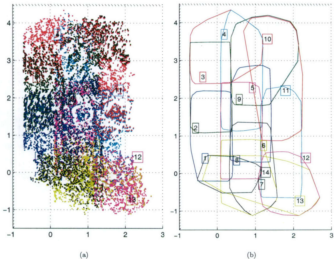
Figure 5-16: Plan view (xy) of the placement of submaps for the four JHU tracklines in a global frame. (a) features color-coded by submap. (b) The convex hull of the submaps shows high overlap in the temporal sequence and varying degrees of overlap across track.
