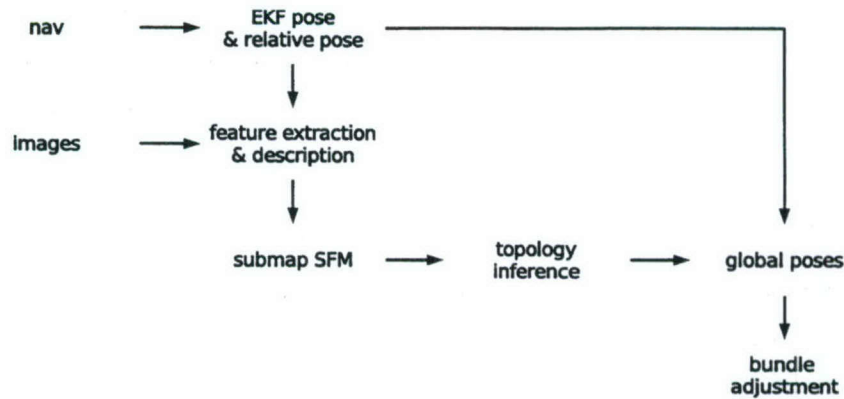
Figure 1-5: Flowchart of structure and motion recovery from underwater imagery. An image sequence is processed into short submaps of structure and motion aided by navigation information. Submaps are then matched to infer and refine additional spatial constraints (such as loop closures and parallel tracklines). An initial guess of poses and structure in a global frame is then used to perform a final bundle adjustment.
