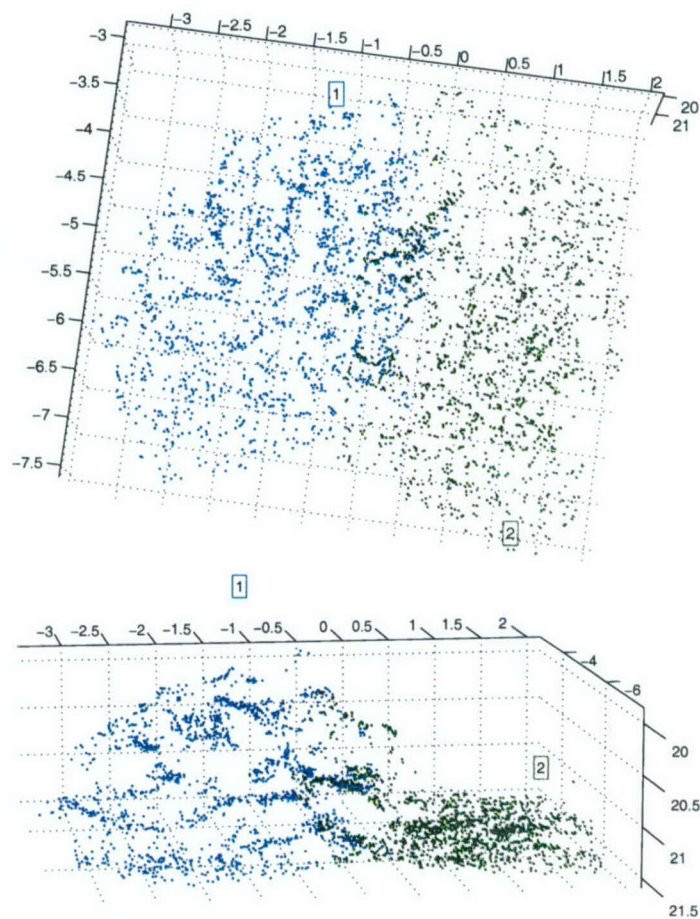
Figure 5-4: Views of the registered submaps that contain the images in figure 5-3. The blue dots correspond to the 3D features of the submap on the first trackline of the survey ( i.e. the images on the left column of figure 5-3). The green dots correspond to features in a submap on the second trackline of the survey ( i.e. images in the right column in figure 5-3).
