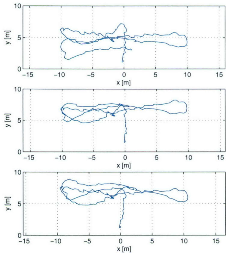
Figure 6-20: (Top) Plane view of the original navigation-based trajectory. (Middle) Image-based trajectory after bundle-adjustment. (Bottom) Corrected navigation-based trajectory.
