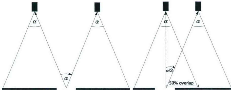
Figure 2-2: Range of viewing angles for an image patch (light gray) given the camera field of view ( \alpha ).
