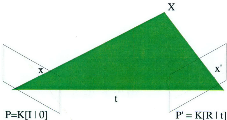
Figure A-2: Two view geometry. The rays \underline{x}, \underline{x}' and \underline{t} form the epipolar plane. This plane intersects the imaging planes in the epipolar lines.
