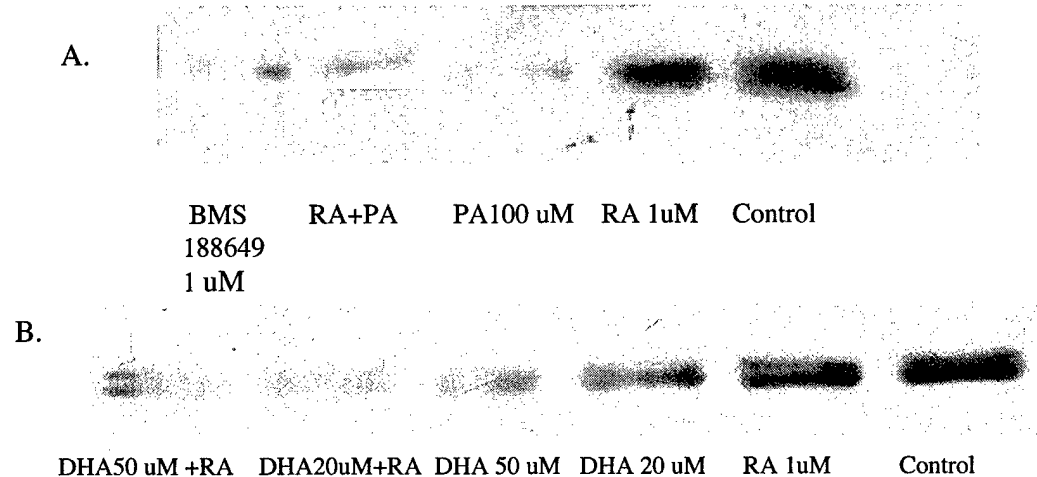
Figure 2. Phytanic acid, DHA, and RXR agonist BMS 188649 inhibited the expression of cyclin D1 in prostate cancer PC-3 cells. PC-3 cells were seeded in 10-cm dishes. Cells were treated with various drugs for 48 hours. Cells were harvested and the whole cell lysate protein was extracted for Western blot.
