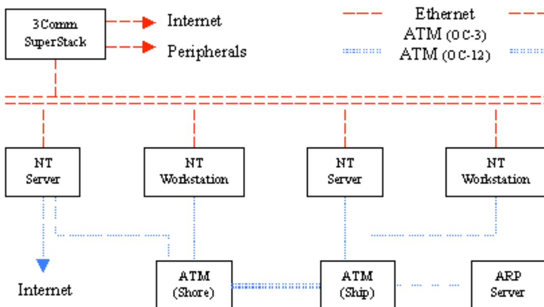
Figure 1. Core ATM and Ethernet Networking Connections
