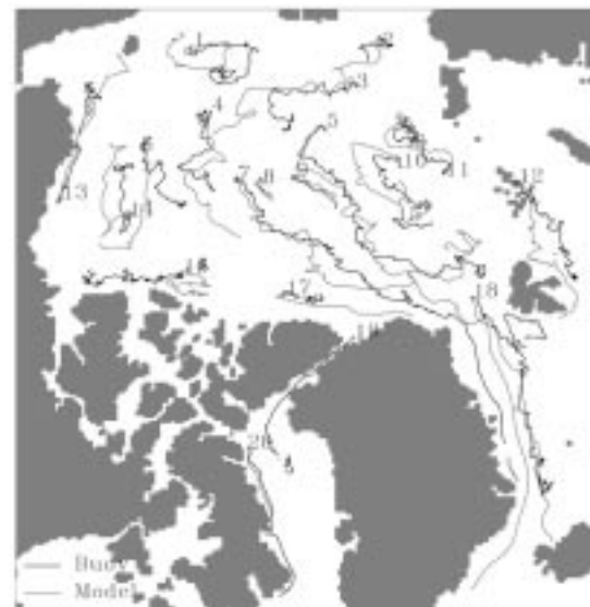
Figure 2: Trajectories of drifting buoys deployed on Arctic sea ice during the period 1990-1994, compared with simulated tracks from a sea-ice model. The model was driven by observed atmospheric data of the same time period and by simulated ocean currents.
