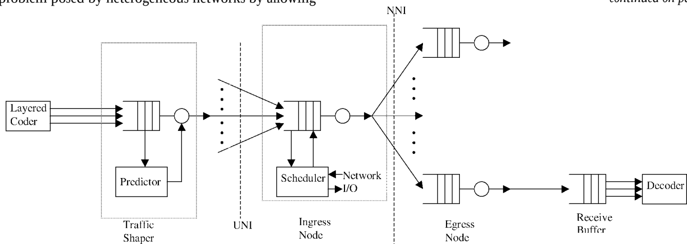
Figure 2. Specific elements for delivering layered video over ATM networks.
