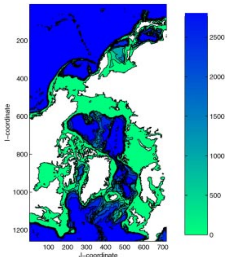
Figure 6. Domain of the new Polar Ice Prediction System, showing the 1280x720 grid for 9-km horizontal spacing and also the 40-level depiction of model depths (m).
