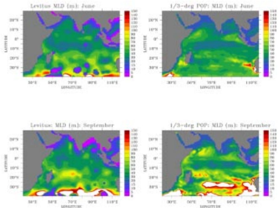
Figure 5. Mixed-layer depths (m) in the Indian Ocean from climatology (left) and as simulated (right). Judging from the months of June and September, the model better depicts Monsoon-induced depth changes than a climatology derived from sparse data.
