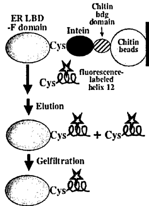
Fig. 3 Fluorescence-labeling of ER by protein splicing. This strategy requires a C-terminally truncated fragment of the ER \beta LBD that lacks the F-domain and H12. This ER \beta fragment is linked via a cysteine residues to a modified splicing domain of the yeast protein intein. This fusion protein can be purified by binding to chitin beads via a chitin binding domain (CBD) that has been engineered at the C-terminus of the intein domain. In the presence of free thiols the linkage between the ER domain and intein is cleaved. In our case, the free thiol is at the N-terminal end of a synthetically synthesized and fluorescence-labeled H12. Hence breaking the linkage between the ER LBD domain and intein will result in linking the labeled helix at the C-terminus of the ER LBD. Upon elution of the labeled ER LBD from the chitin column, free H12 peptides are removed by gel filtration.
