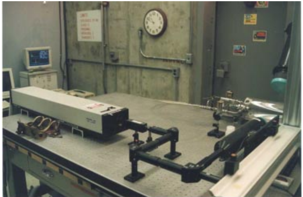
Phase Doppler Particle Analyzer
