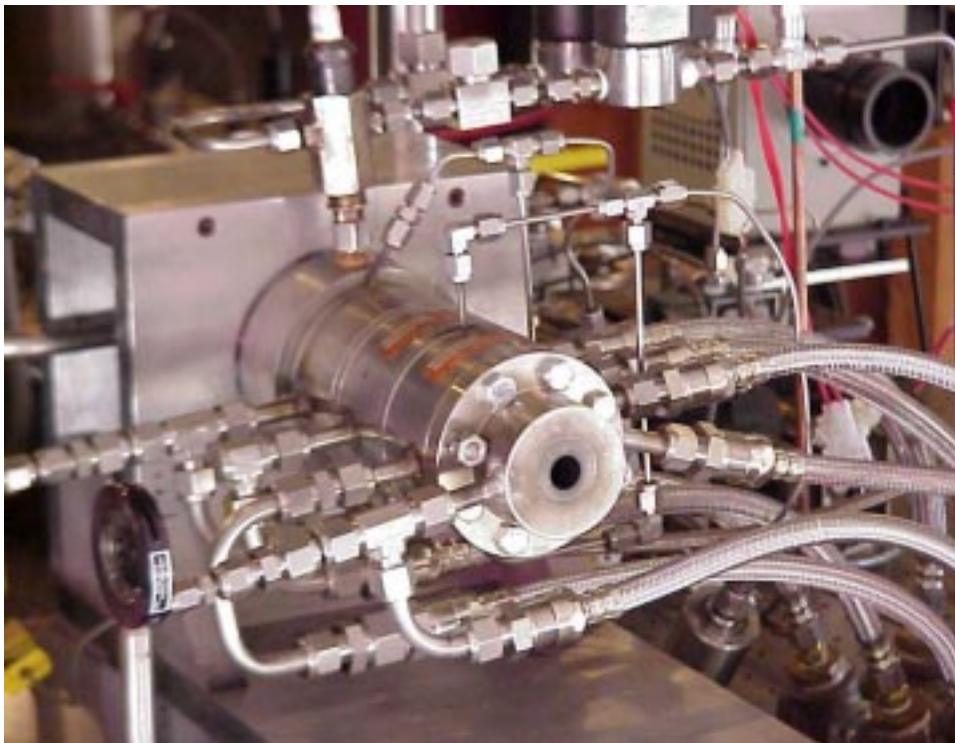
Above: Labscale Liquid-Fuel Rocket Engine
