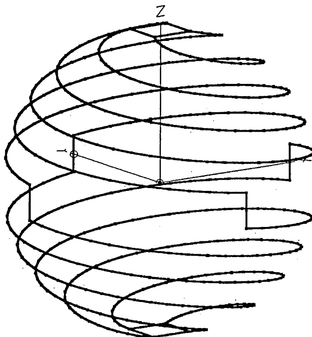
Figure 5. Depiction of the elliptically polarized, electrically small, 4-arm folded spherical helix antenna. The antenna has an overall length of 8.36 cm and is resonant at 301.3 MHz with a resistance of 61.5 Ohms.
