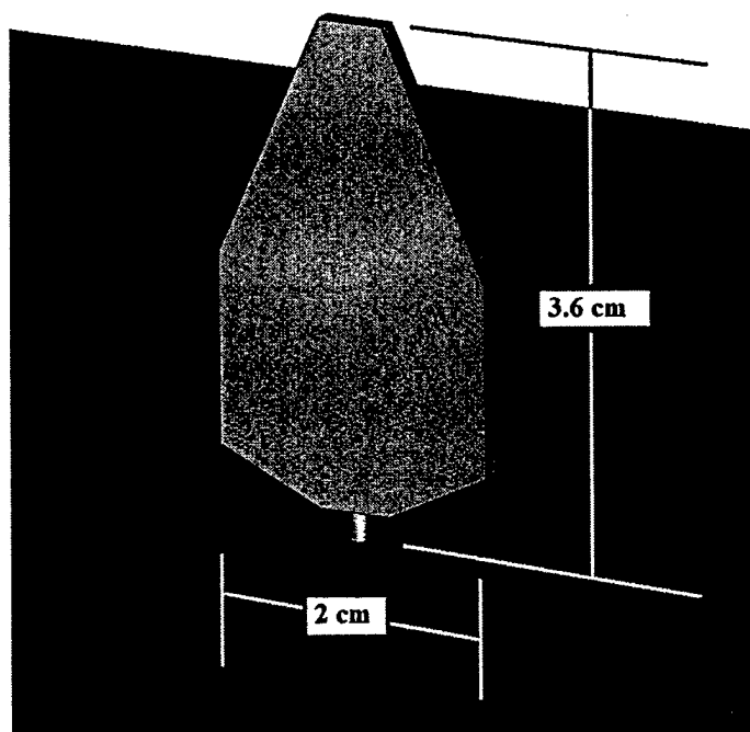
Figure 2. Depiction of a simple planar monopole antenna having a height of 3.6 cm and a width of 2 cm. This planar monopole antenna has a 2:1 VSWR bandwidth in excess of 7.5:1.
