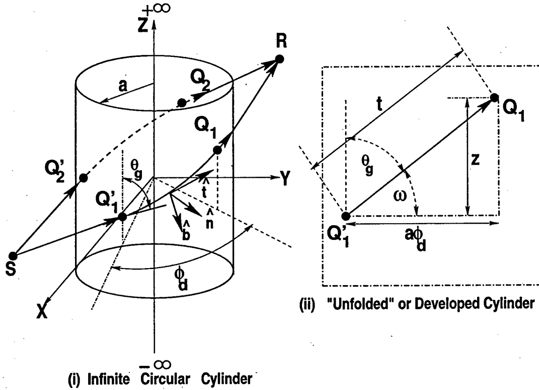
Fig. 2. Scattering by a perfectly conducting circular cylinder in terms of two dominant creeping wave (ray) paths. The unfolded cylinder corresponds to the high-frequency planar limit when ka \rightarrow \infty . The moving trihedron (along the geodesic path length, t , for Q_1' \rightarrow Q_1 ) is defined by the unit vectors, \hat{b} (binormal), \hat{n} (normal) and \hat{t} (tangent) such that, \hat{n} = \hat{b} \times \hat{t} . For source S \rightarrow Q_1' , and, R \rightarrow Q_1 , is the canonical case for mutual coupling between antennas on a smooth convex surface, and, \theta_g \rightarrow 0 defines the paraxial region. The general topology shown here applies to the calculation of shadowing of wing-mounted antennas by the aircraft/missile fuselage. A special case of this scenario is shown explicitly in Fig. 3, below.
