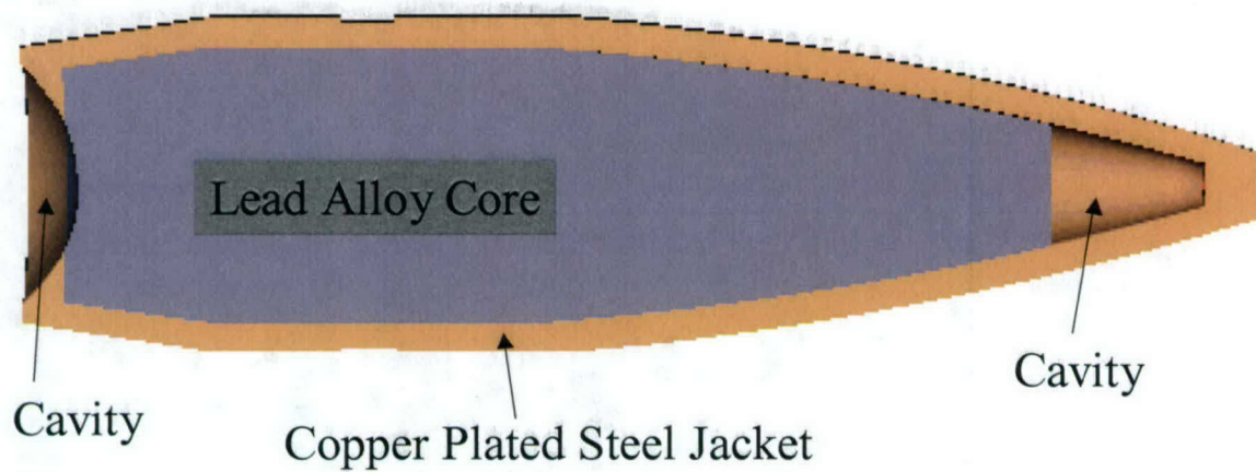
Figure 10 7.62 mm M80 projectile
