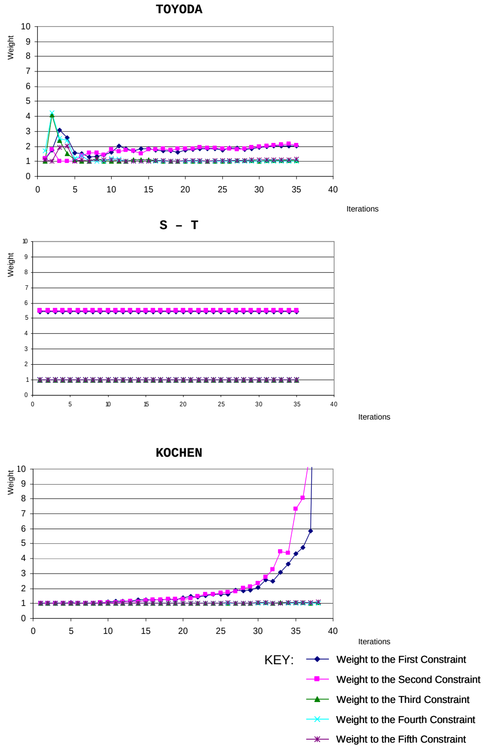
Figure 14. Performance of Weight Trend of Legacy Heuristics for Setting (1,1,2,2,2)
