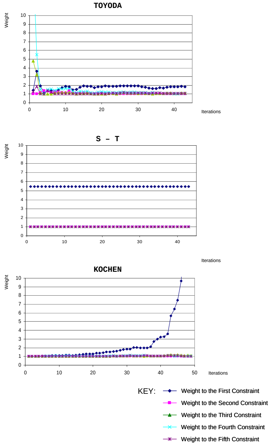
Figure 15. Performance of Weight Trend of Legacy Heuristics for (1,2,2,2,2)
