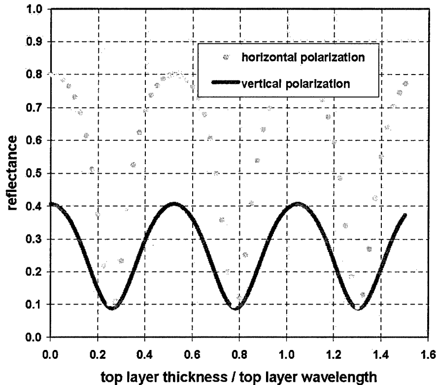
Figure 10. Oblique incidence reflectance from a dielectric coating over water ( \epsilon = 9 )
