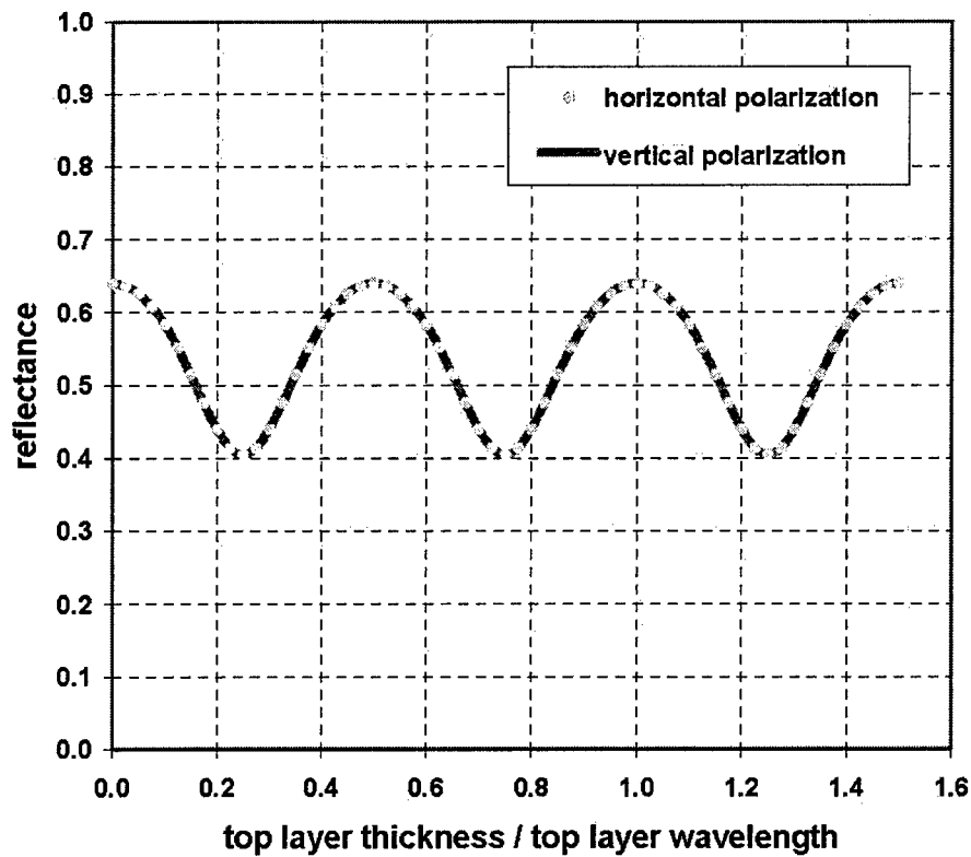
Figure 8. Normal incidence reflectance from a dielectric coating over water ( \epsilon = 2 )
