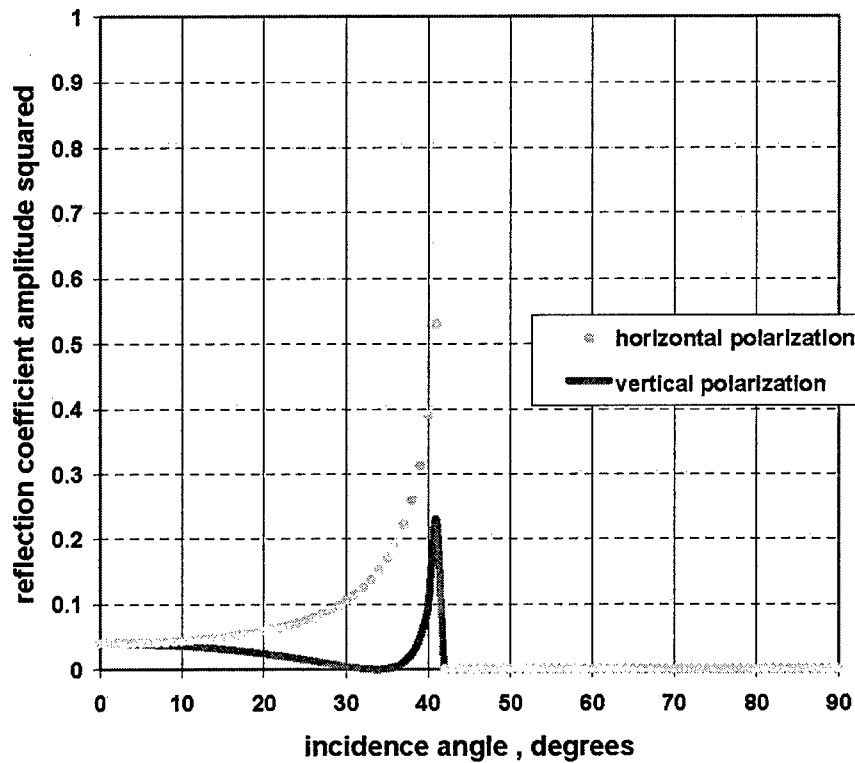
Figure 6. Reflectance from a glass-air interface (total internal reflection)
