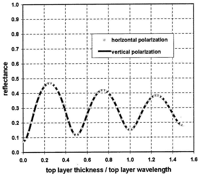
Figure 23. Reflectance from a low-loss moist layer at normal incidence
