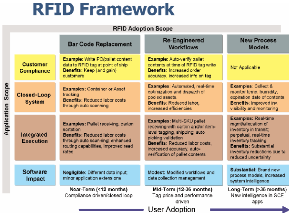
Figure 8: RFID Framework
