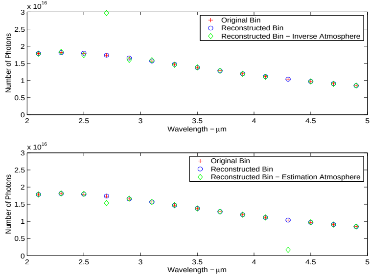
Figure 5.31: This figure shows the sum of photons in each wavelength bin for the 1600^{\circ}K fireball in the reconstructed data compared with the original data cube. The sum of photons for the reconstruction of atmospherically attenuated detector data is also shown.
