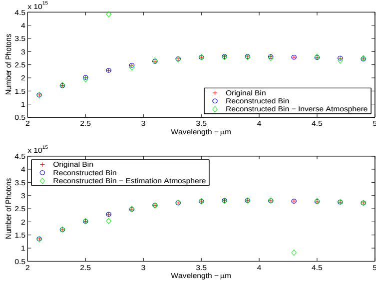
Figure 5.29: This figure shows the sum of photons in each wavelength bin for the 1000^{\circ}K fireball in the reconstructed data compared with the original data cube. The sum of photons for the reconstruction of atmospherically attenuated detector data is also shown for both atmospheric reconstruction methods.
