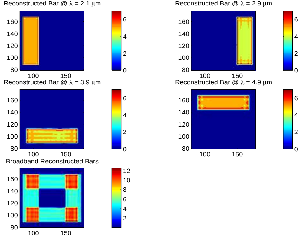
Figure 5.15: This figure shows the reproduction of the original overlapping bar test data cube by the 2D reconstruction algorithm. The bar test consists of four monochromatic sources in four spectral bins. The original sources have a uniform five photons across their extent with the remaining bins containing zero photons. The final subplot shows a total 2 - 5\mu m view of the reproduced data.
