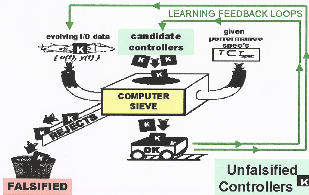
Figure 3: The unfalsification process mathematically sifts controllers to find those that are consistent with both performance goals and physical data. It plays the role of a ‘supervisor’ that chooses one of the currently unfalsified controllers to put in the aircraft’s control loop.
