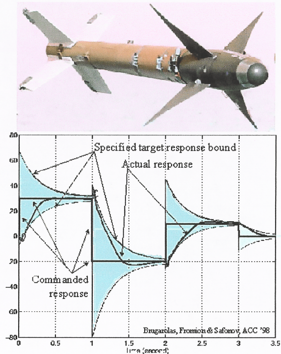
Figure 4: A data-driven unfalsified missile controller would have abilities to adaptively discover solutions in real-time to compensate for sudden in-flight changes and damage.
