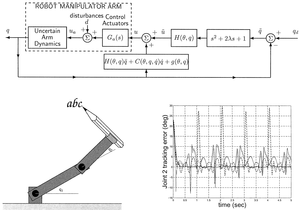
Figure 5: Unfalsified control produced superior results for a nonlinear two-link robot manipulator subject to uncertain dynamics, noisy disturbances and abrupt changes in load mass. The two sluggishly smooth traces large amplitude signals in the plot are with a conventional adaptive controller used to adjust control gain-vector \theta(t) , and the two very low amplitude traces are for the unfalsified controller. The unfalsified controller had a much quicker, sure-footed and precise response without increased control effort.
