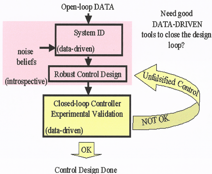
Figure 1: The data-driven theory of unfalsified control closes data-driven portion of the design loop by focusing squarely and precisely on the control design implications of data.
