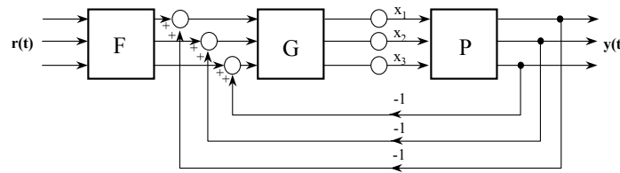
Figure 37: MIMO Control Structure for a Three-by-Three System (3x3).
