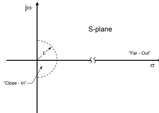
Figure 51: Right-half-Plane Analysis.
