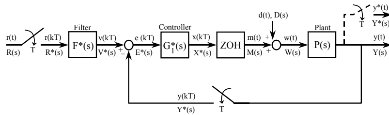
Figure 29: A MISO Sampled-data Control System.
