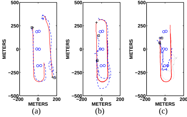
Figure 5: Estimated tracks: (a) Scenario 1, (b) Scenario 2 for the two end targets, and (c) Scenario 2 for the middle targets. In the figures, the dotted and dashed lines represent MM-JPDA and MM-PDA tracks, respectively.
