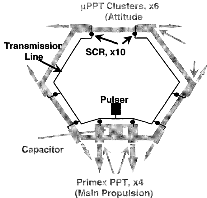
Figure 2 Propulsion Module
