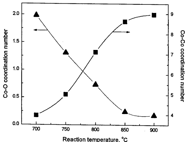
Fig. 12. Coordination numbers of the first Co–O and Co–Co shells as a function of reaction temperature, as fitted from the EXAFS spectra.
