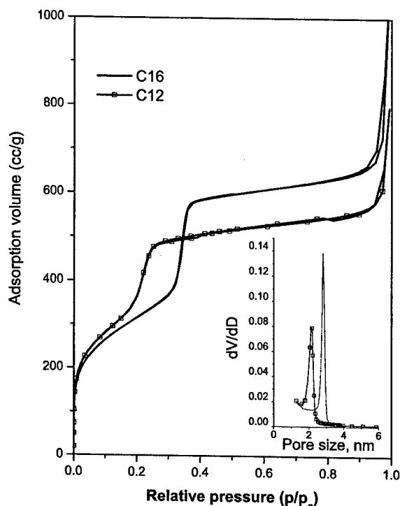
Figure 1. Physorption isotherms measured with fresh C12 and C16 templates. The inset shows the pore size distribution derived from the desorption isotherms by the modified BJH method. 31
