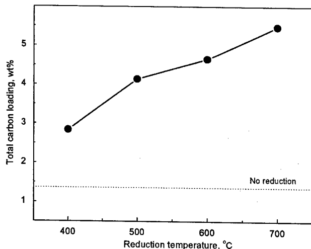
Fig. 3. The carbon yield as a function of the catalyst prerduction temperature.
