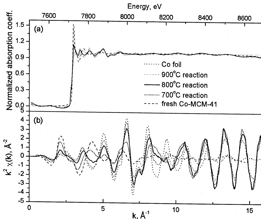
Fig. 9. EXAFS data for Co-MCM-41 catalysts after reaction at different temperatures. The fresh Co-MCM-41 and the cobalt foil are given as references. (a) Normalized EXAFS data calibrated relative to the cobalt foil. (b) The k^2 -weighted EXAFS data in the k space.
