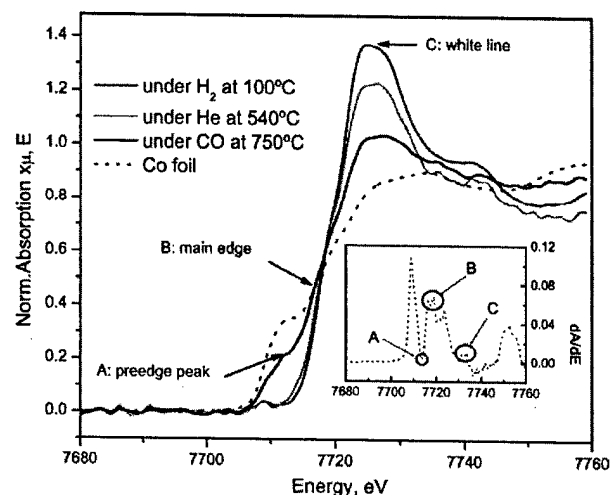
Figure 2. The XANES region of the EXAFS spectra recorded for Co-MCM-41 under different atmospheres and for the cobalt foil reference. The inset shows the energy values corresponding to the pre-edge peak (A), main edge energy (B), and white line (C) as determined from the first derivative of the EXAFS spectrum recorded for the Co foil. The maximum intensity of the EXAFS spectrum recorded for the Co-MCM-41 samples is shifted to lower energy compared to that observed for the Co foil ( \sim 7730 eV).
