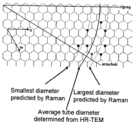
Figure #2. Distribution of SWNT diameters determined for SWNT grown in Co-MCM-41 with pores of 2.85nm. The background mesh represents the graphene sheet and the colored dots indicate the individual semiconducting tubes identified in our sample by fluorescence measurements. The straight solid lines represent the axes for wrapping the carbon net to form zigzag or armchair nanotubes. Data from DNA wrapping suggests 2 main tubes. Reaction at higher pressure will likely narrow the distribution.
