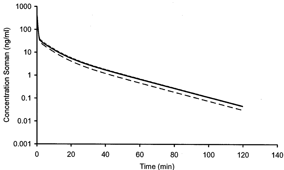
Figure 27 Predicted concentration (ng/mL) of C(+)-P(-)-soman and C(-)-P(-)-soman in blood of guinea pigs after i.v. bolus administration of a dose of C(±)P(±)-soman corresponding with 6 LD50 (165 µg/kg). Solid lines naive animal, dashed lines HuBuChE-pretreated animal.
