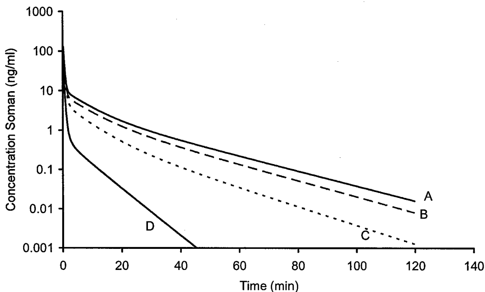
Figure 28 Calculated concentration (ng/mL) of C(+)-P(-)-soman and C(-)-P(-)-soman in blood of guinea pigs after i.v. bolus administration of a dose of C(±)P(±)-soman corresponding with 2 LD50 (55 µg/kg). Naive animals: A: C(-)-P(-)-soman, B: C(+)-P(-)-soman; HuBuChE-pretreated animals: C: C(-)-P(-)-soman, D: C(+)-P(-)-soman
