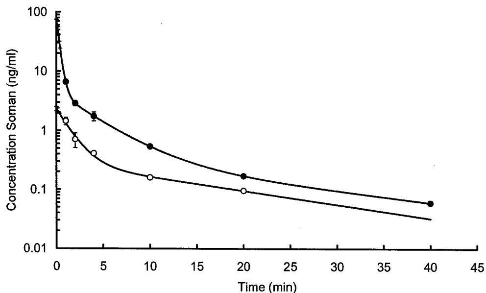
Figure 3 Mean concentration (ng/mL) \pm SEM of C(+)-P(-)-soman ( \circ ) and C(-)-P(-)-soman ( \bullet ) in blood of individual anesthetized, atropinized and mechanically ventilated guinea pigs after i.v. bolus administration of a dose of C( \pm )-P( \pm )-soman corresponding with 2 LD50 (55 \mu g/kg).
