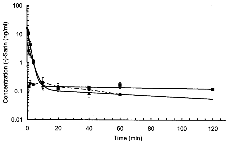
Figure 31 Mean concentration-time course of (-)-sarin (ng/mL \pm SEM, n=4) in blood of anesthetized, atropinized and mechanically ventilated guinea pigs after i.v. administration of a ( \pm )-sarin dose of 48 \mu g/kg, which corresponds with 2 LD 50 . Naive animals (■), HuBuChE-pretreated animals 1, 4 (▲), HuBuChE-pretreated animals 2, 3, 5 (●).
