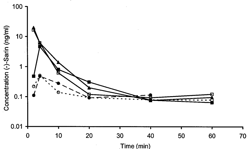
Figure 16 Concentration-time courses of (-)-sarin (ng/mL) in blood of anesthetized and atropinized guinea pigs after a 2-min nose-only exposure to 200 \text{ mg}\cdot\text{m}^{-3} of ( \pm )-sarin vapor in air. ○ = guinea pig GP 12, ■ - guinea pig GP 15, ● = guinea pig GP 16, □ = guinea pig GP 18, ▲ = guinea pig GP 21.
