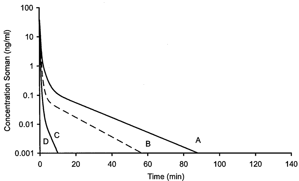
Figure 29 Predicted concentration (ng/mL) of C(+)-P(-)-soman and C(-)-P(-)-soman in blood of guinea pigs after i.v. bolus administration of a dose of C( \pm )-P( \pm )-soman corresponding with 2 LD50 (55 \mu g/kg). Naive animals: A: C(-)-P(-)-soman, B: C(+)-P(-)-soman; HuBuChE-pretreated animals: C: C(-)-P(-)-soman, D: C(+)-P(-)-soman.
