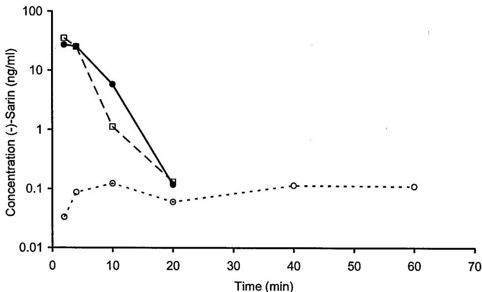
Figure 15 Concentration-time courses of (-)-sarin (ng/mL) in blood of anesthetized, atropinized, and HuBuChE-pretreated guinea pigs after a 2-min nose-only exposure to 376 \text{ mg}\cdot\text{m}^{-3} of ( \pm )-sarin vapor in air. \circ = guinea pig GP 9, \bullet = guinea pig GP 10, \square = guinea pig GP 11.
