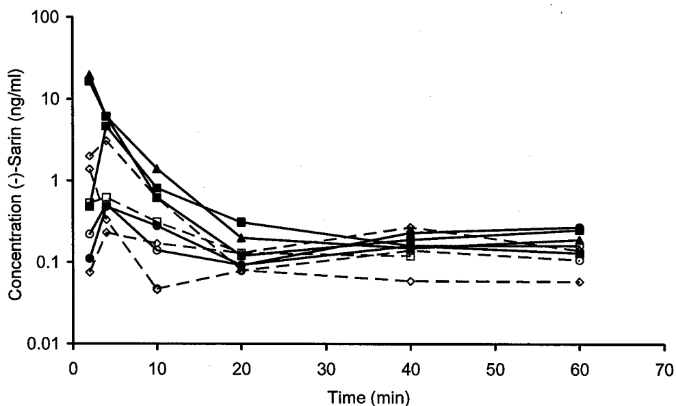
Figure 32 Concentration-time courses of (-)-sarin (ng/mL) in anesthetized and atropinized guinea pigs after a 2-min nose-only exposure to 200 \text{ mg}\cdot\text{m}^{-3} (±)-sarin vapor in air. HuBuChE-pretreated animals: open markers, dotted lines; non-pretreated animals: filled markers, solid lines
