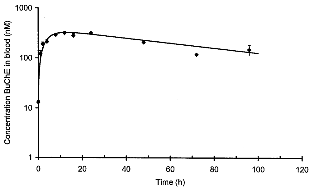
Figure 18 Concentration-time course of BuChE-activity measured in blood of marmosets (n=3), following intramuscular administration of HuBuChE (35 nmol). Data were fitted to the following equation: [BuChE] = 390 \cdot \exp(-0.013 \cdot t) - 377 \cdot \exp(-0.2554 \cdot t) .
