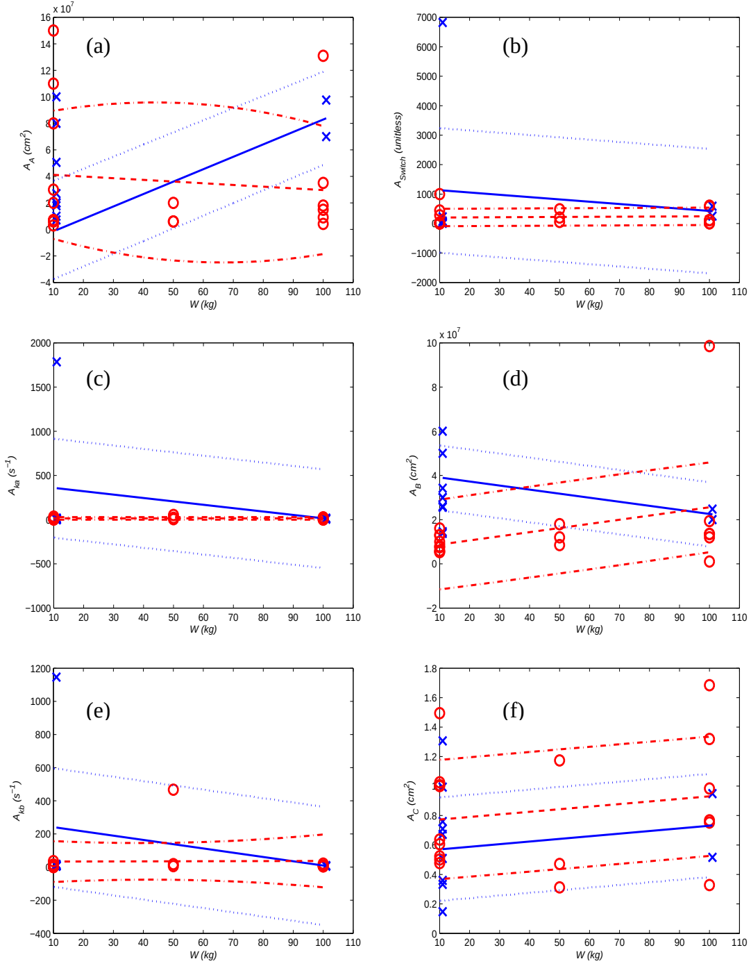
Figure 122. Potential scaling relationships exhibit fireball area features dependence upon weight ( W ). Figures (a) through (f) contain the spectral features for A_A , A_{\text{Switch}} , A_{ka} , A_B , A_{kb} , and A_C .
