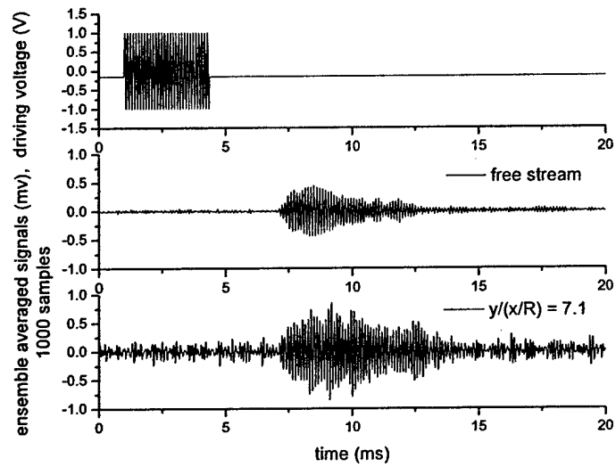
Figure 9. Boundary layer response to the free stream acoustic forcing: x = 4.25'' , R = 483 , f = 8.9\text{kHz} , 30 waves.
