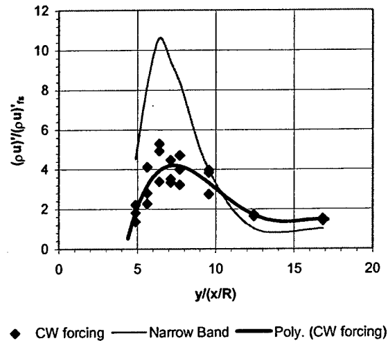
Figure 5. Non-dimensional amplitude distribution in the boundary layer with continuous forcing compared with the "naturally occurring" case, f = 8.9 \text{ kHz} , R = 700 .
