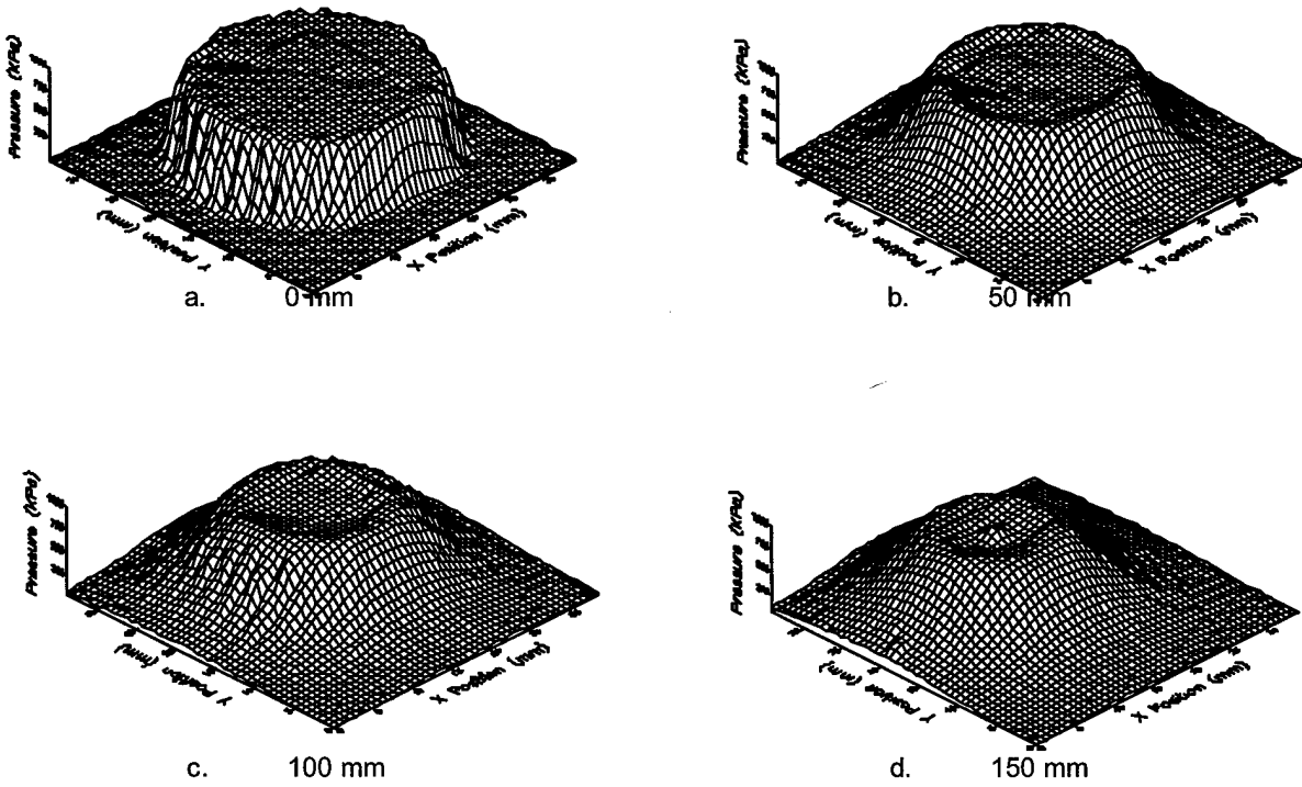
Figure 15 Transducer Pressure Variations with Distance
