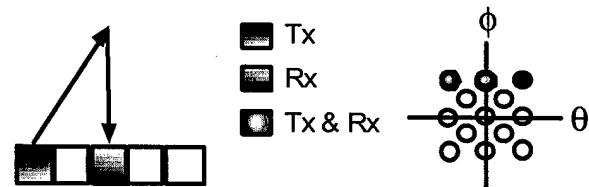
Figure 4. SAAS TAA geometry. We can acquire k-space data at the same lateral spatial frequencies as the backscatter case but at scattering angles less than 180°.
