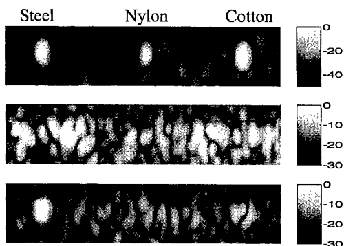
Figure 11. SAAS 180^\circ B-mode image of a 3-wire phantom (top). The middle image is an unsuccessful D-weighted image that is being dominated by the steel wire sidelobes due to psf nonuniformity. The bottom image is a successful D-weighted image highlighting the contrast available in angular scatter imaging.
