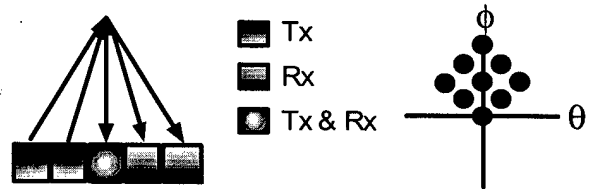
Figure 2. Angular scatter k-space response for a 1D array utilizing multielement apertures and the TAA to maintain system psf.
