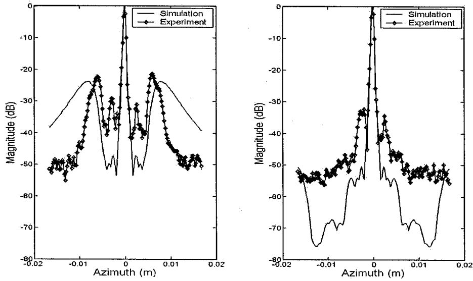
Figure 10: Lateral beamplots for simulation and experimental data showing the reduction of grating lobes achieved when applying the TAA half element step. Acoustic backscatter (left) is combined with the TAA half element step to produce the beamplots on the right.
