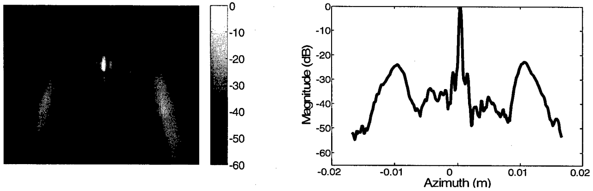
Figure 7. Log compressed 180^\circ SAAS image of a wire target (left) and associated beamplot (right). Sidelobe levels are around -27 dB.
