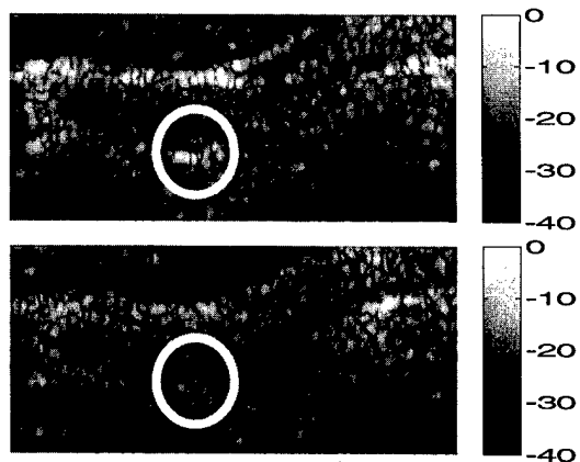
Figure 12. SAAS 180^\circ pure backscatter B-mode image of in vivo human thyroid (top) and a D-weighted image of human thyroid (bottom) between 180^\circ and 176^\circ . Notice the dissipation of the bright scatterer inside the white ring in the D-weighted image.
