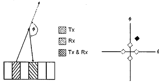
Figure 7: Full element TAA geometry where the algorithm has been applied relative to the backscattered case depicted in Fig. 3. Notice how this setup samples the same lateral spatial frequency as the backscattered case but at a scattering angle that is less than 180^\circ and less than the half element TAA scattering angle.
