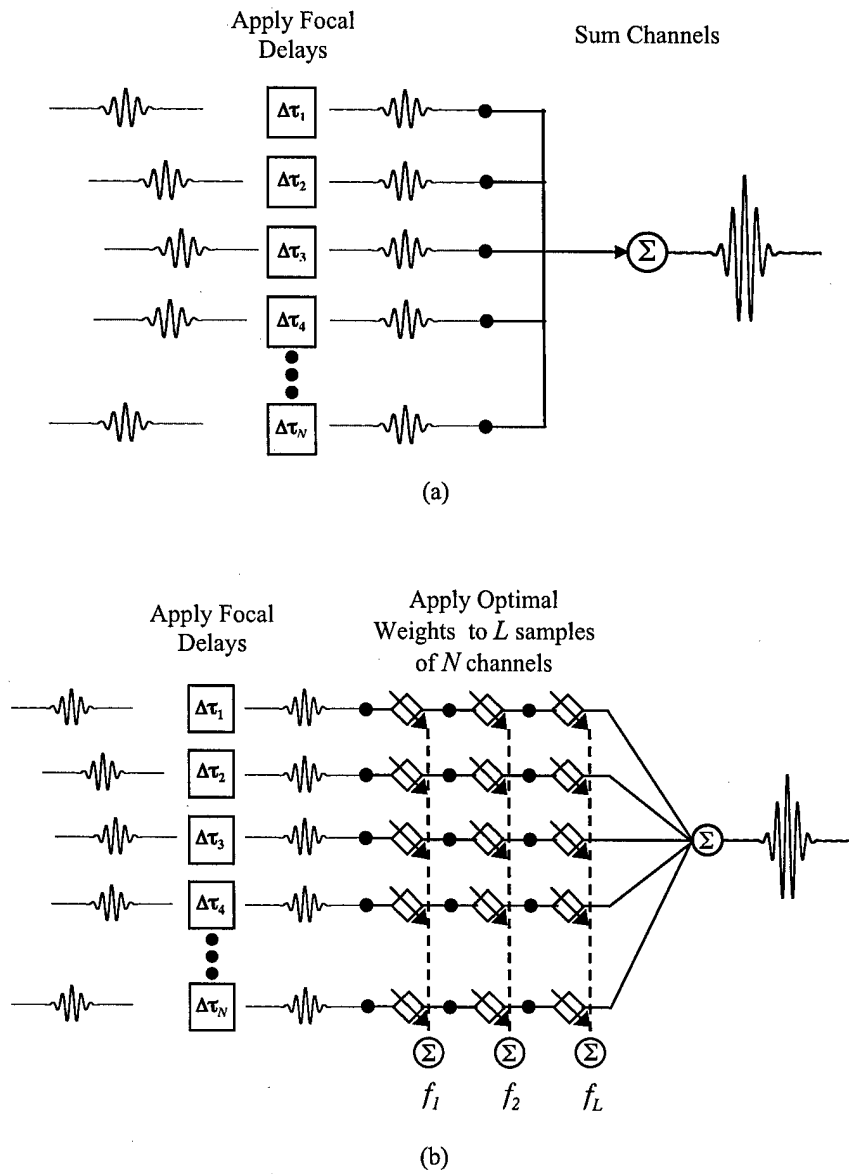
Figure 1. Schematic diagrams of (a) conventional delay-and-sum receive beamformer and (b) constrained adaptive beamformer. Time delays \Delta\tau_i are precalculated for each sample.
