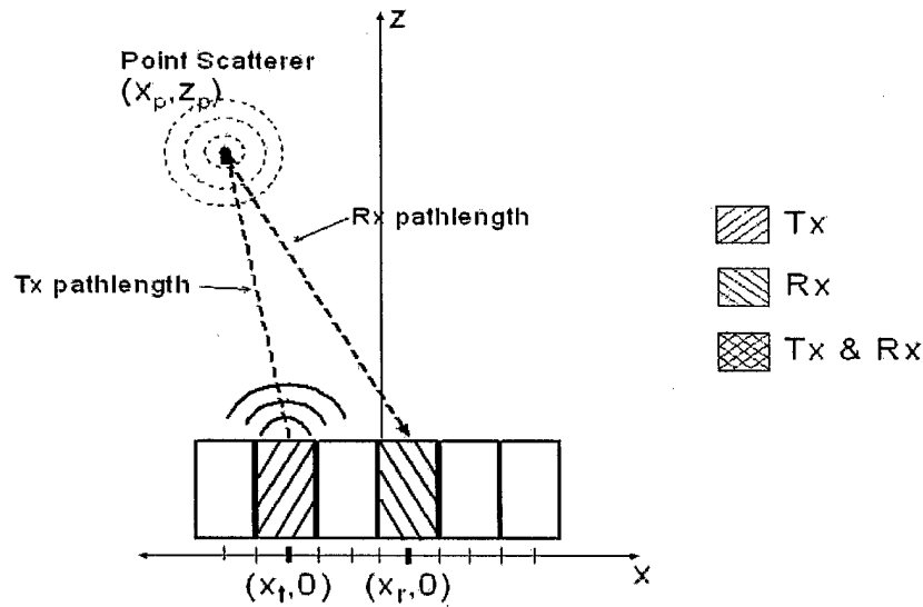
Figure 2: Calculation of propagation times for Single Element Angular Scatterer. The transmit and receive pathlengths are calculated from Pythagorean geometry and divided by the assumed sound velocity through the medium. The lateral positions of the transmit element and receive element are denoted x_t and x_r , respectively. The point (x_p, z_p) is the point at which we focus the received data.
