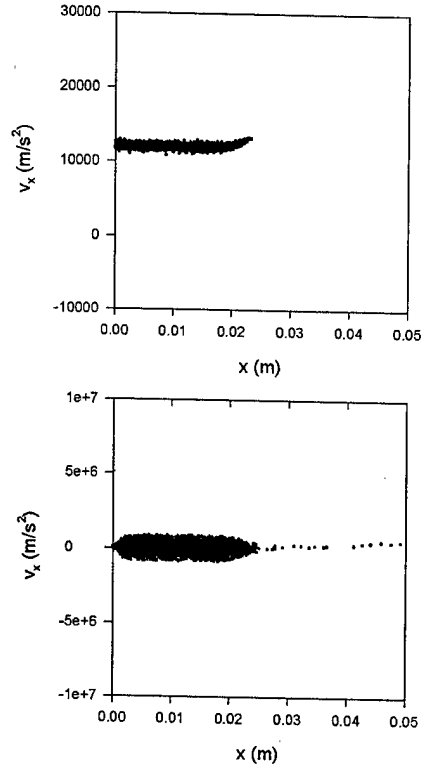
Figure 8: V_x - x phase space for Case 1.4, \tau=1.8E-6 s. Top: ions, bottom: electrons.
