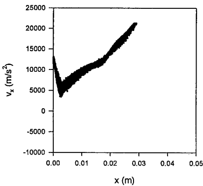
Figure 11: V_x - x phase space of ions for Case 2.3. \tau=1.8E-6 s
