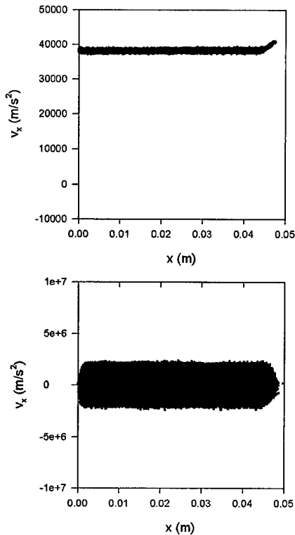
Figure 9: V_x - x phase space for Case 1.5. \tau=1.2E-6 s. Top: ions, Bottom: electrons.
