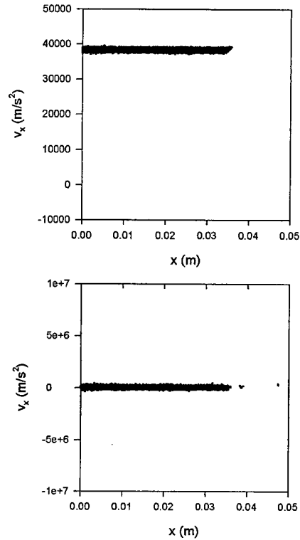
Figure 10: V_x - x phase space for Case 1.6, \tau=1.2e-6 s. Top: ions, Bottom: electrons
