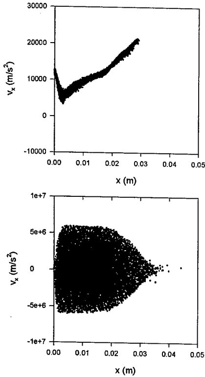
Figure 7: V_x - x phase space for Case 1.3, \tau=1.8E-6 s. Top: ions, bottom: electrons.
